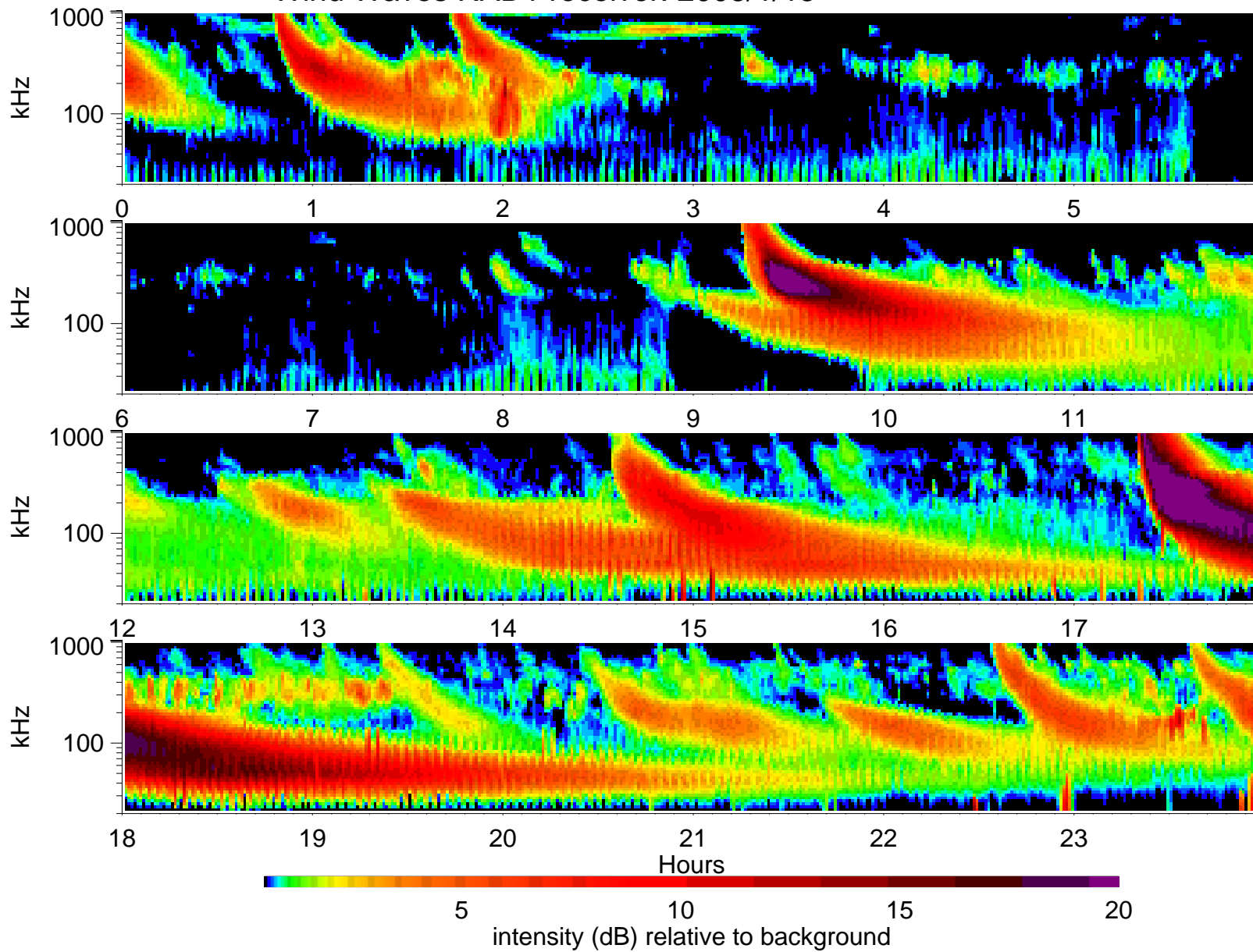
Wind Waves RAD1 receiver: 2003/1/15
