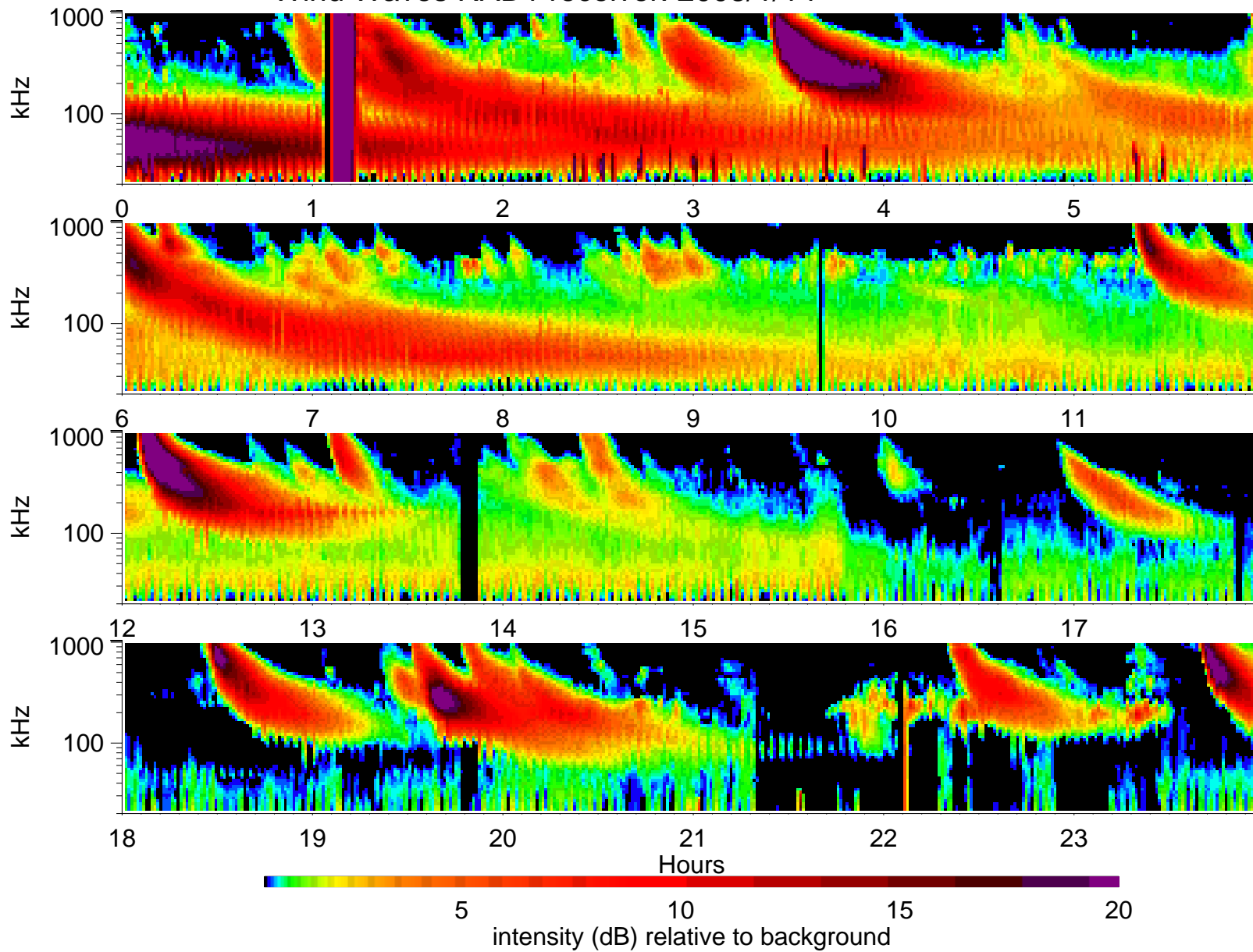
Wind Waves RAD1 receiver: 2003/1/14
