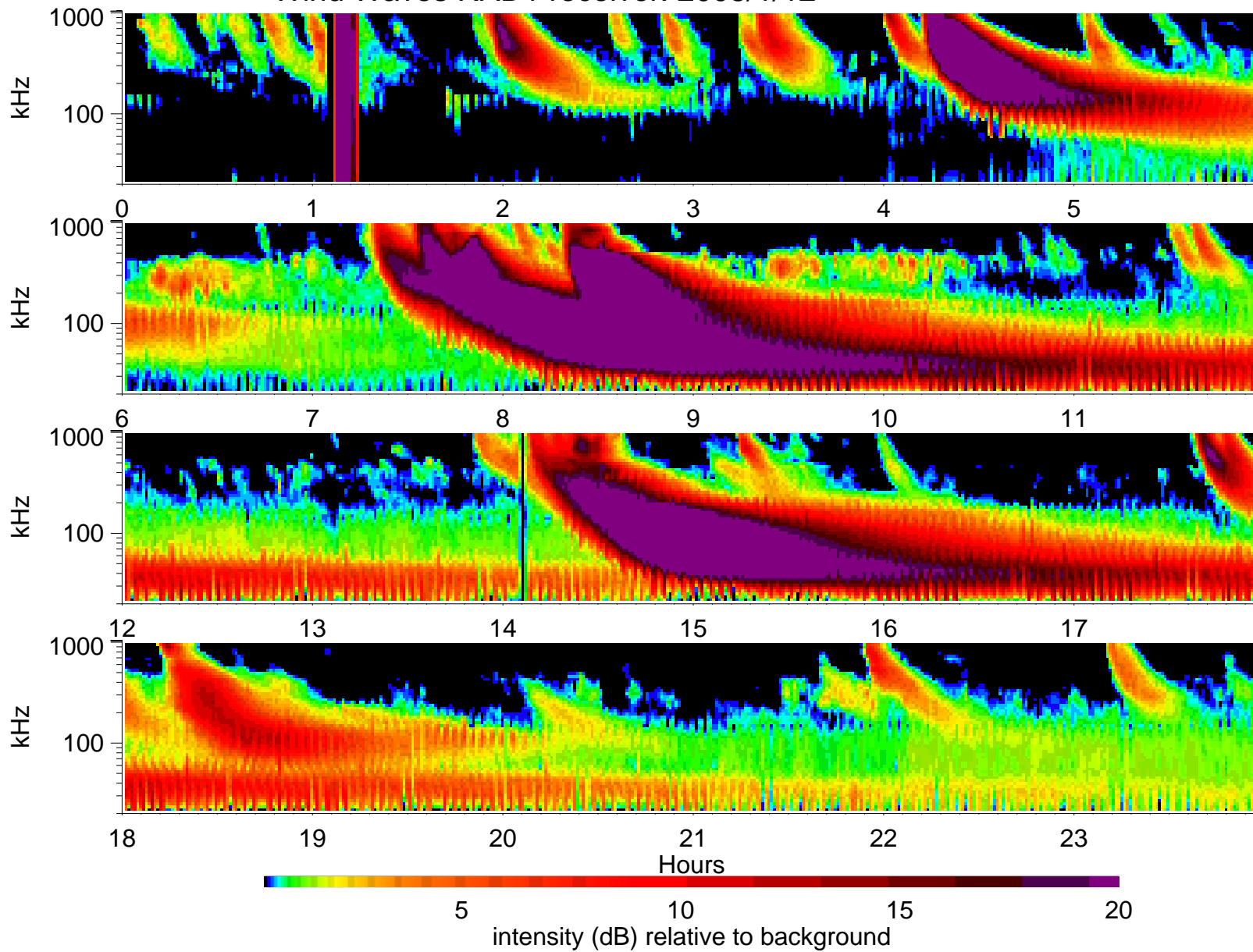
Wind Waves RAD1 receiver: 2003/1/12
