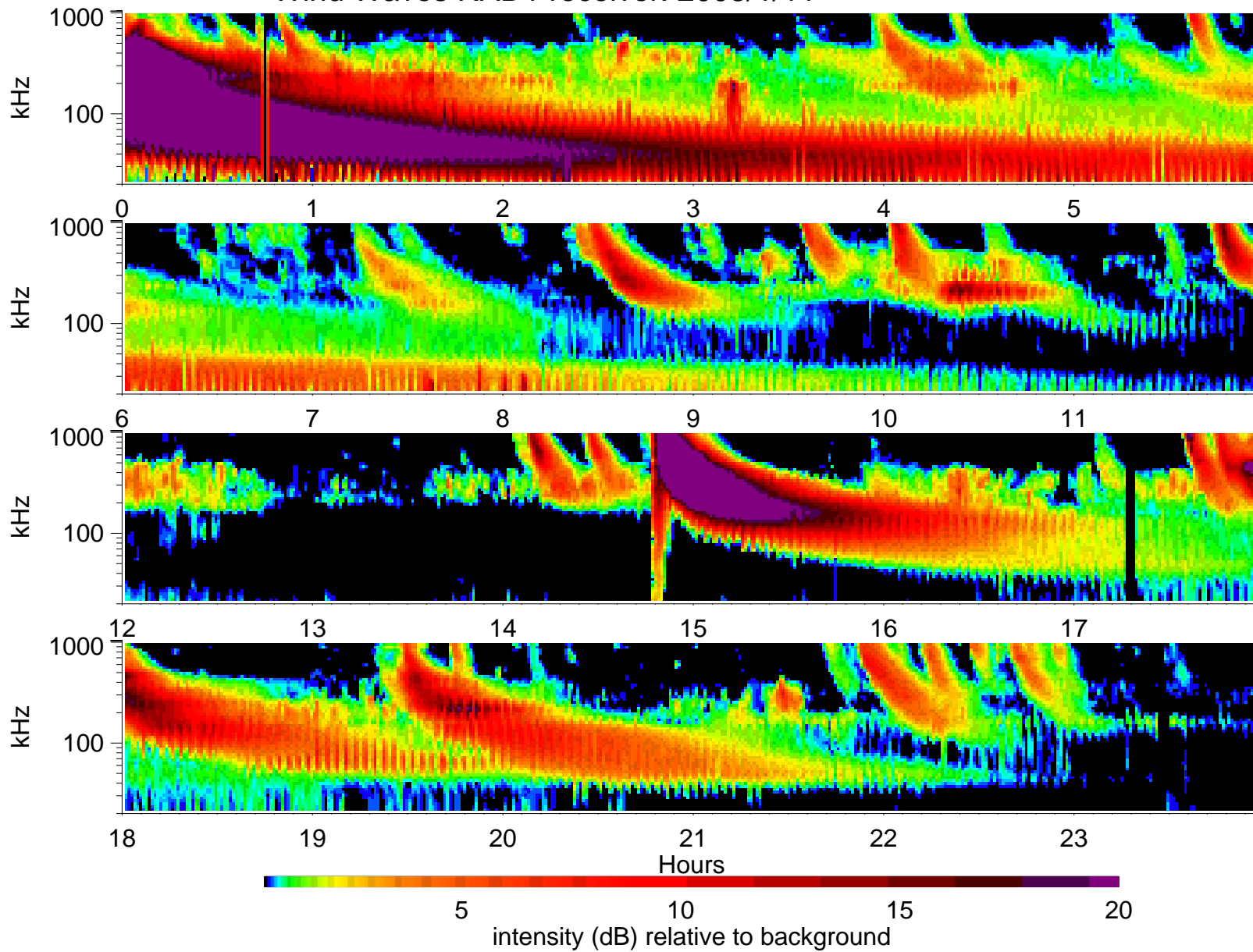
Wind Waves RAD1 receiver: 2003/1/11
