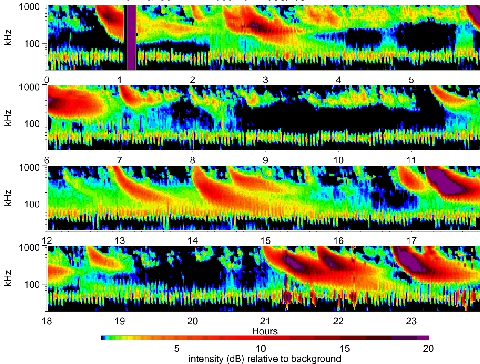
Wind Waves RAD1 receiver: 2003/1/8
