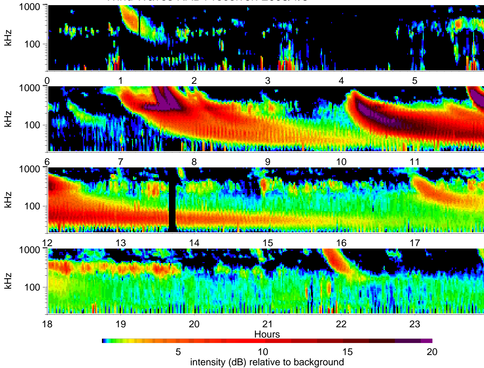
Wind Waves RAD1 receiver: 2003/1/5
