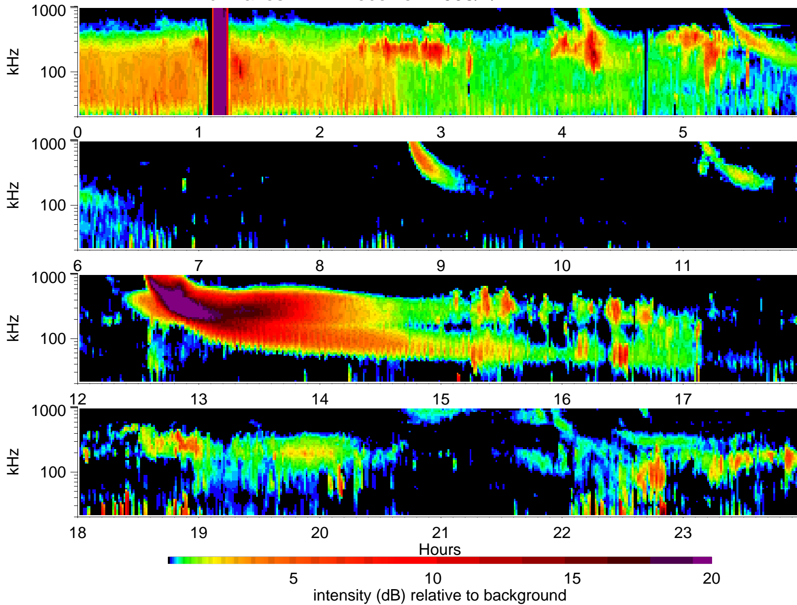
Wind Waves RAD1 receiver: 2003/1/4
