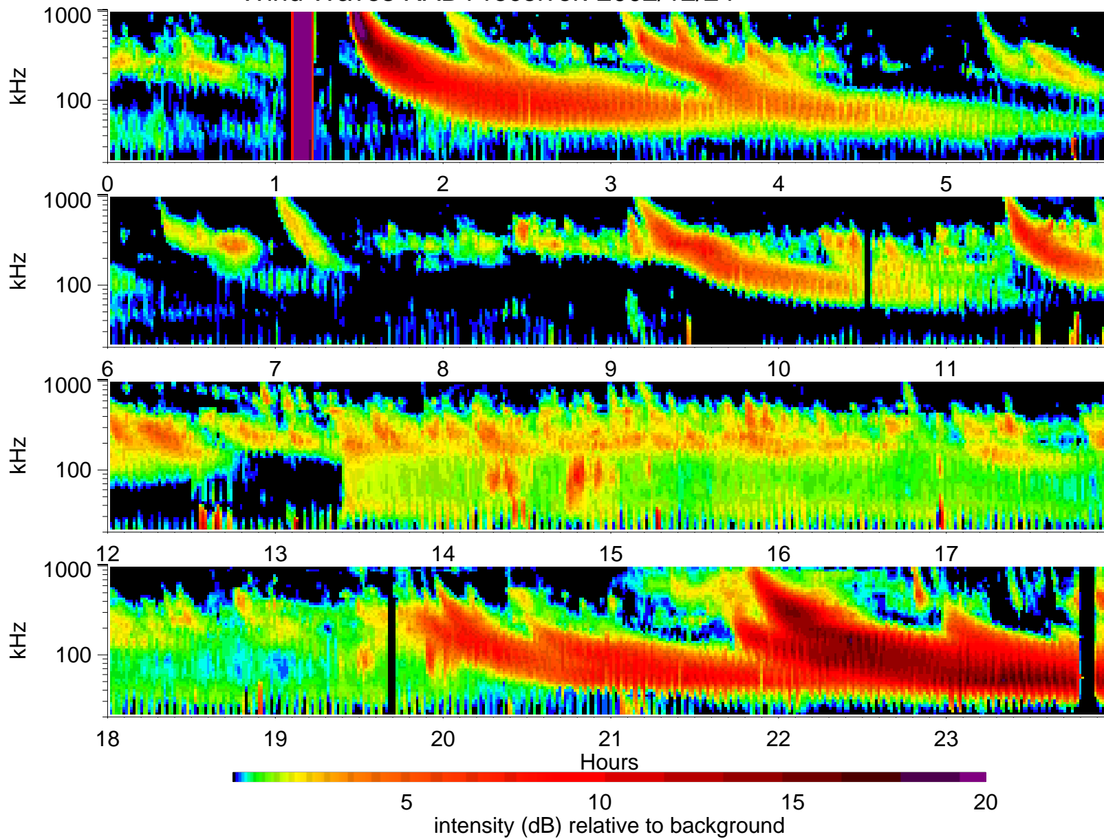
Wind Waves RAD1 receiver: 2002/12/24
