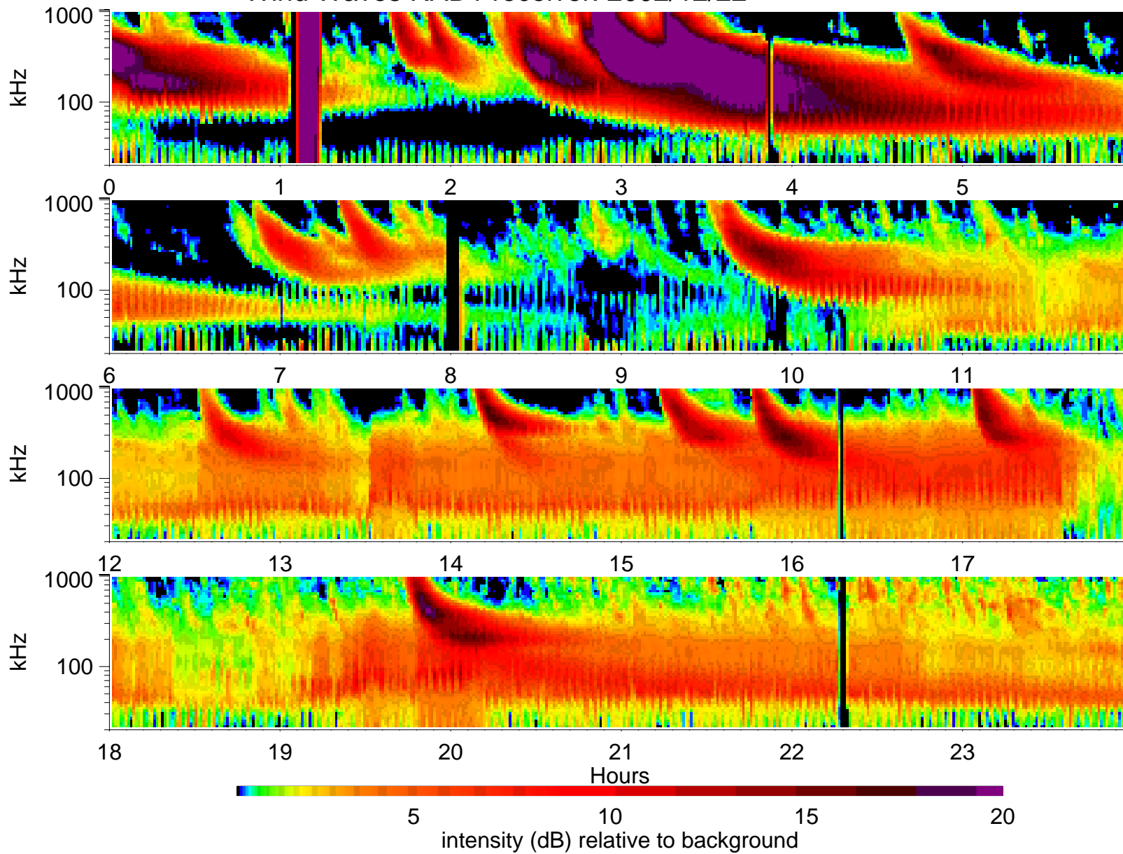
Wind Waves RAD1 receiver: 2002/12/22
