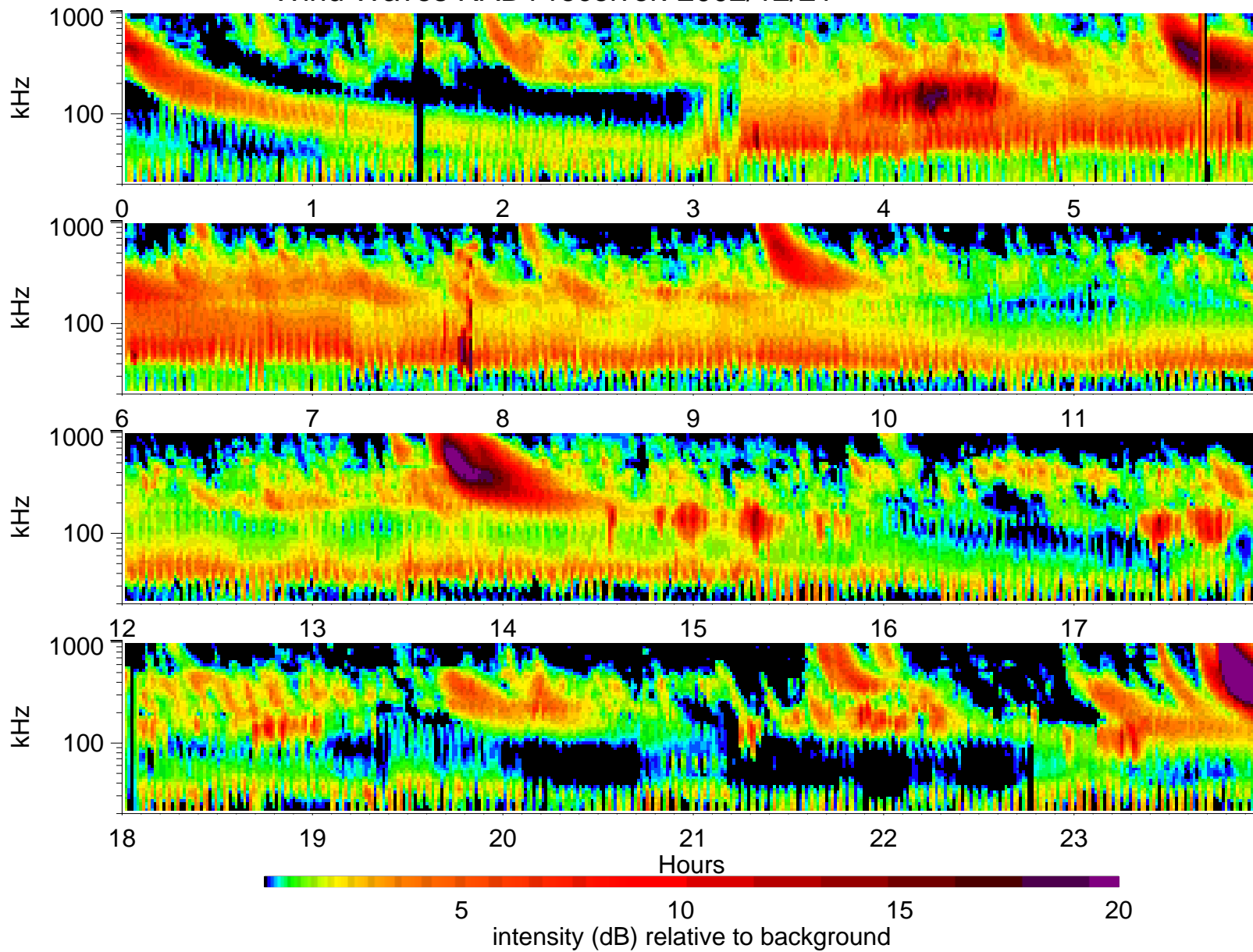
Wind Waves RAD1 receiver: 2002/12/21
