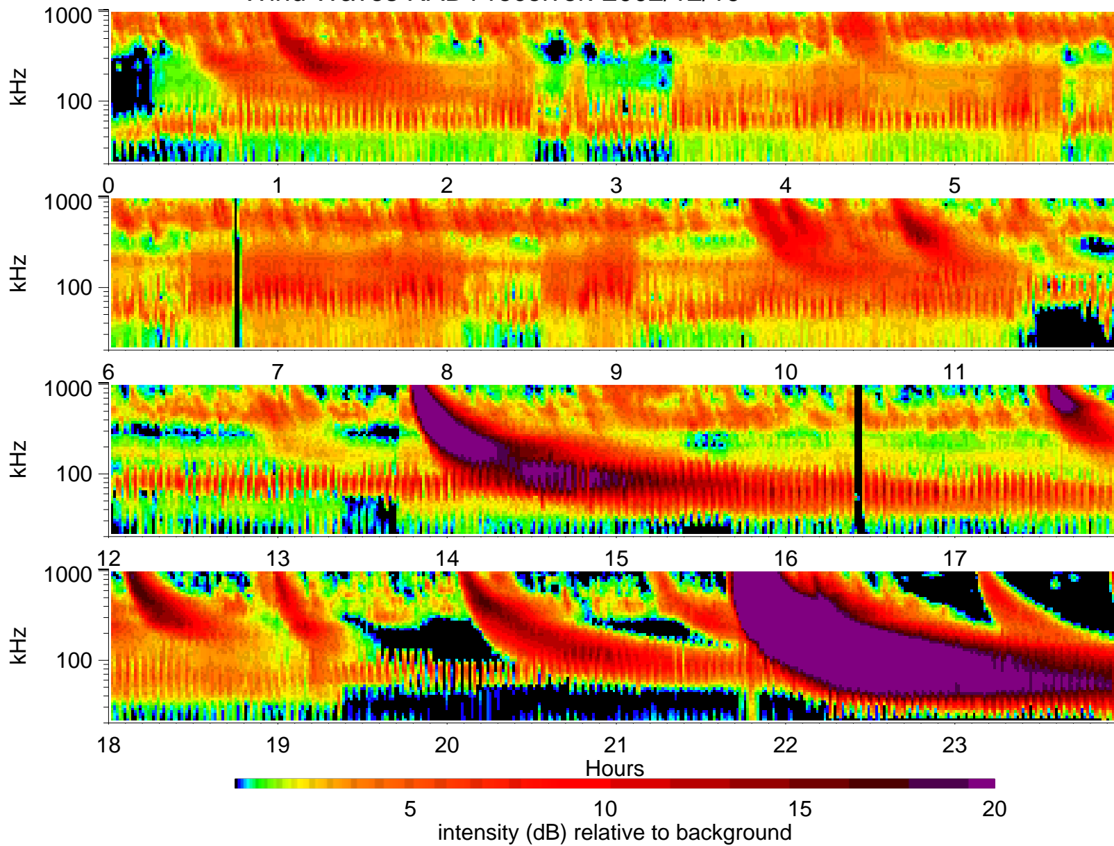
Wind Waves RAD1 receiver: 2002/12/19
