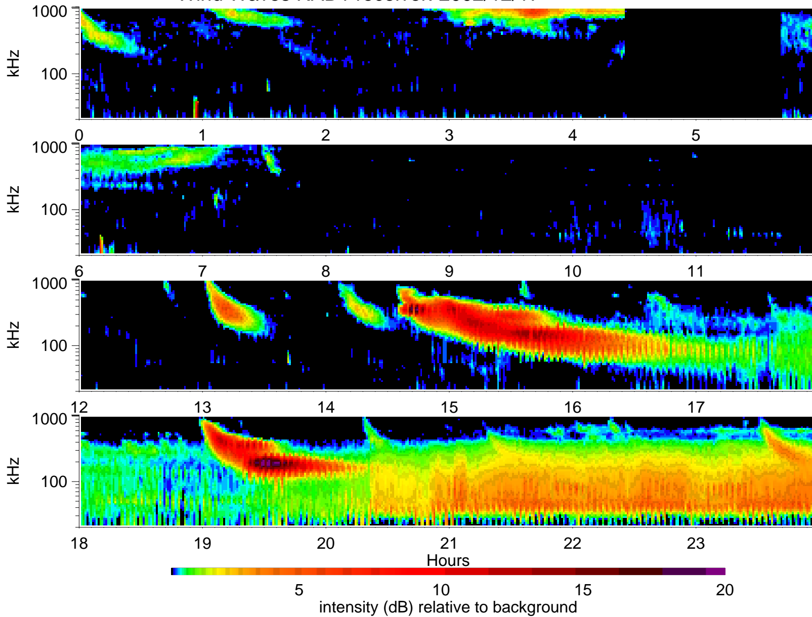
Wind Waves RAD1 receiver: 2002/12/17
