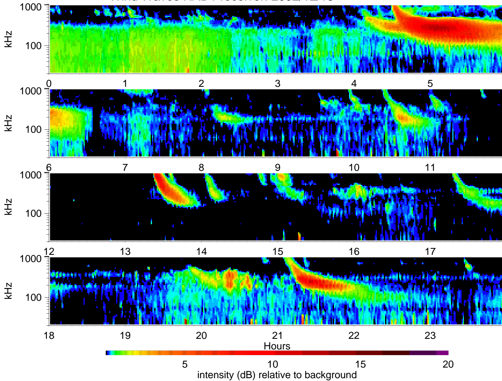
Wind Waves RAD1 receiver: 2002/12/15
