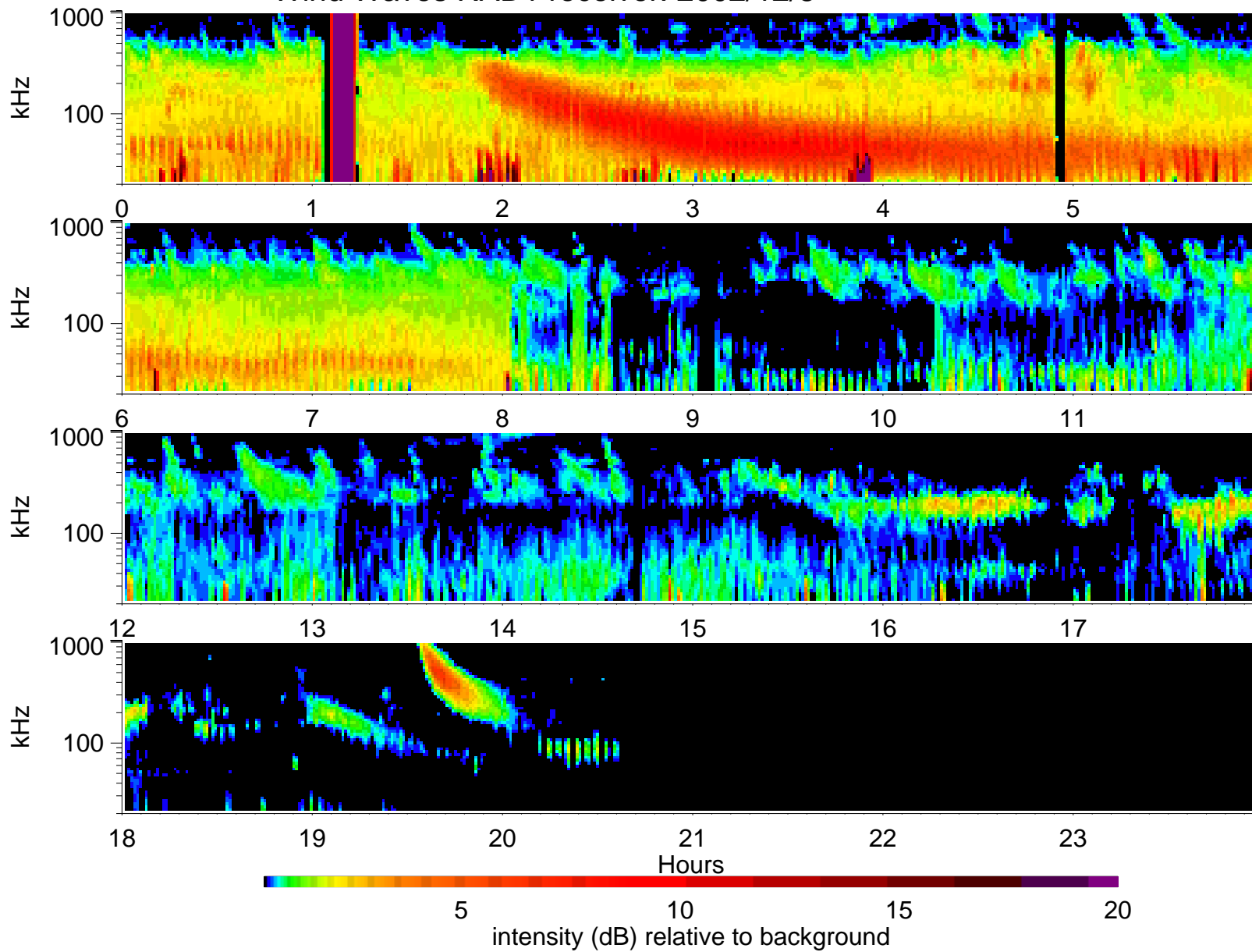
Wind Waves RAD1 receiver: 2002/12/8
