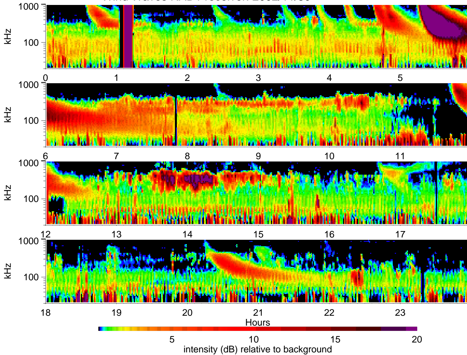
Wind Waves RAD1 receiver: 2002/11/30
