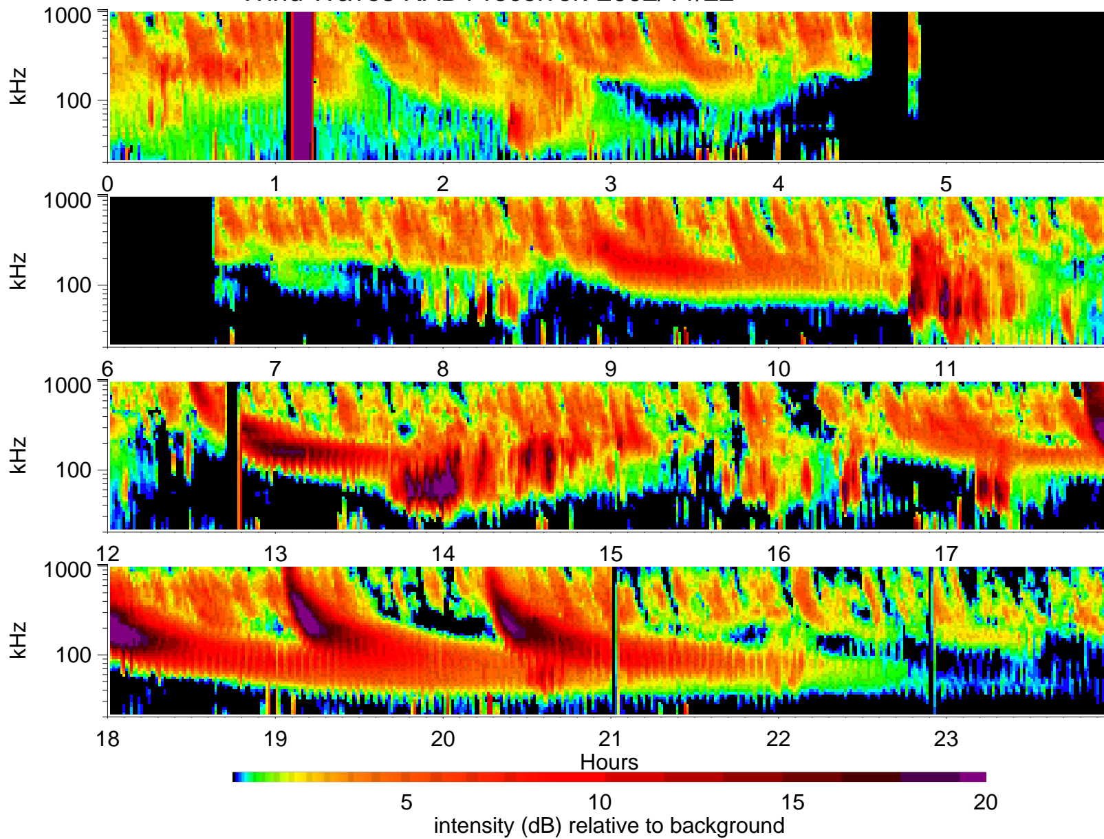
Wind Waves RAD1 receiver: 2002/11/22
