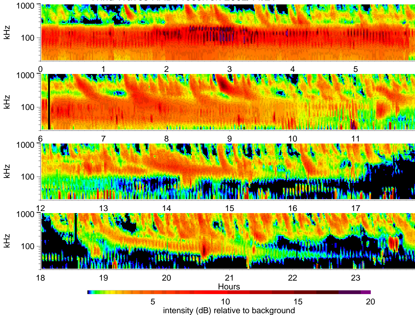
Wind Waves RAD1 receiver: 2002/11/21
