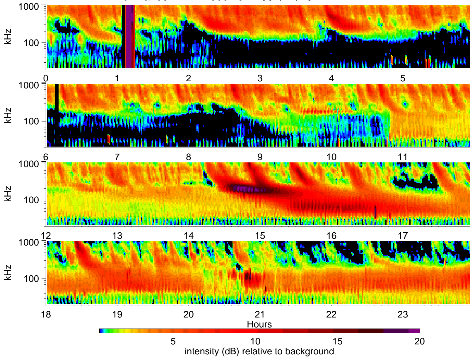
Wind Waves RAD1 receiver: 2002/11/20
