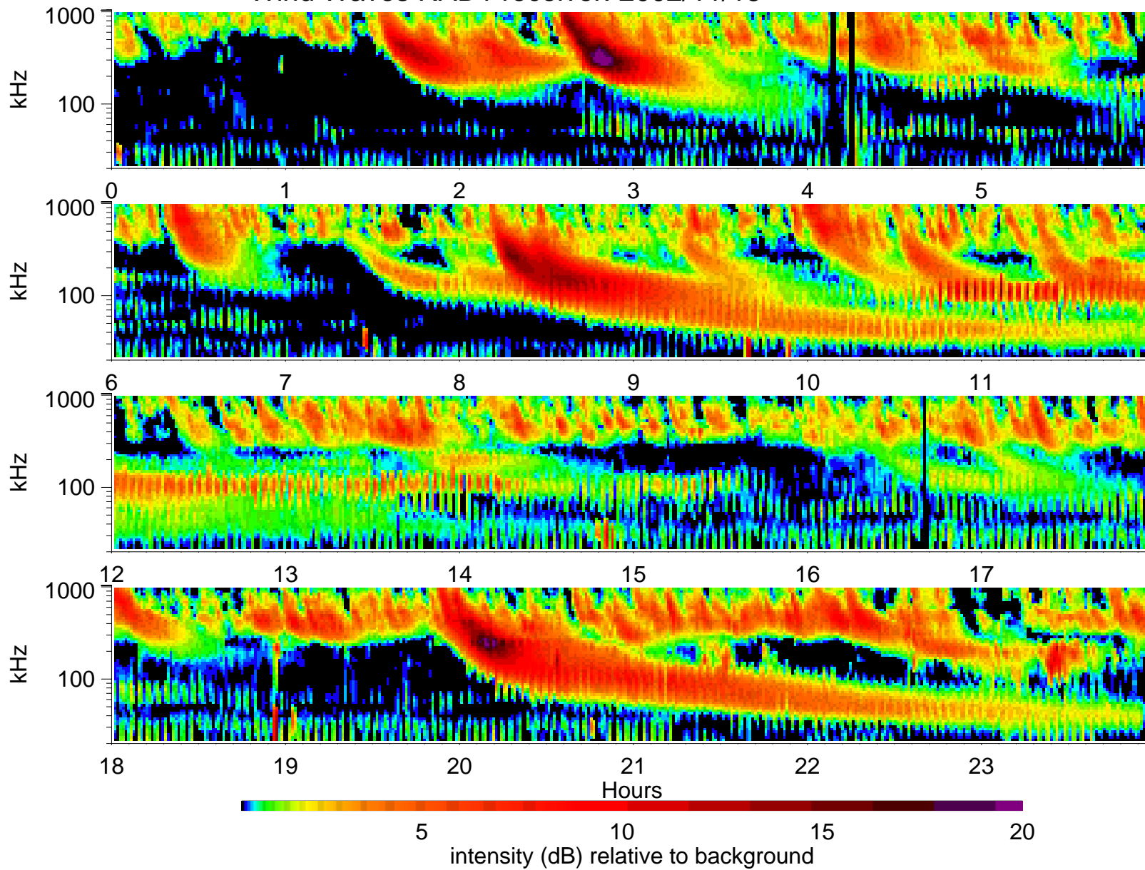
Wind Waves RAD1 receiver: 2002/11/15
