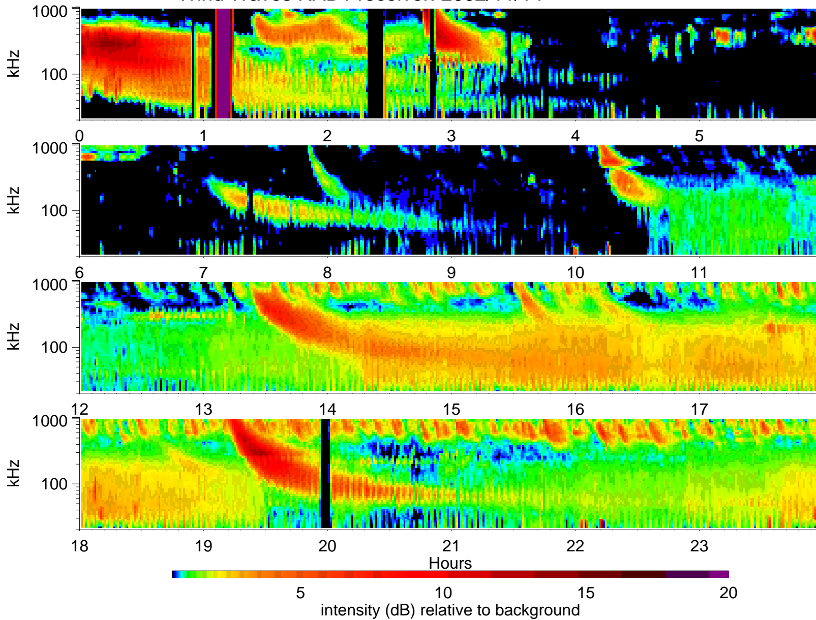
Wind Waves RAD1 receiver: 2002/11/14
