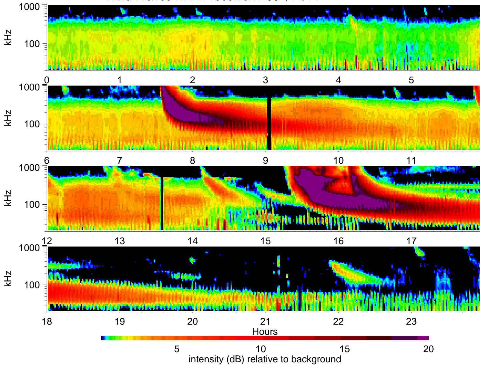
Wind Waves RAD1 receiver: 2002/11/11
