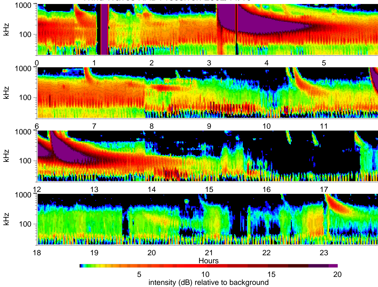
Wind Waves RAD1 receiver: 2002/11/10
