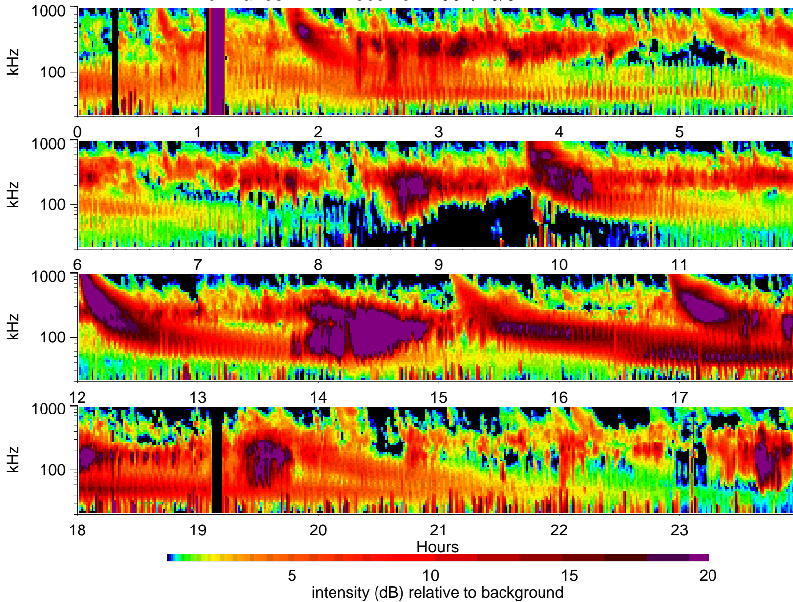
Wind Waves RAD1 receiver: 2002/10/31
