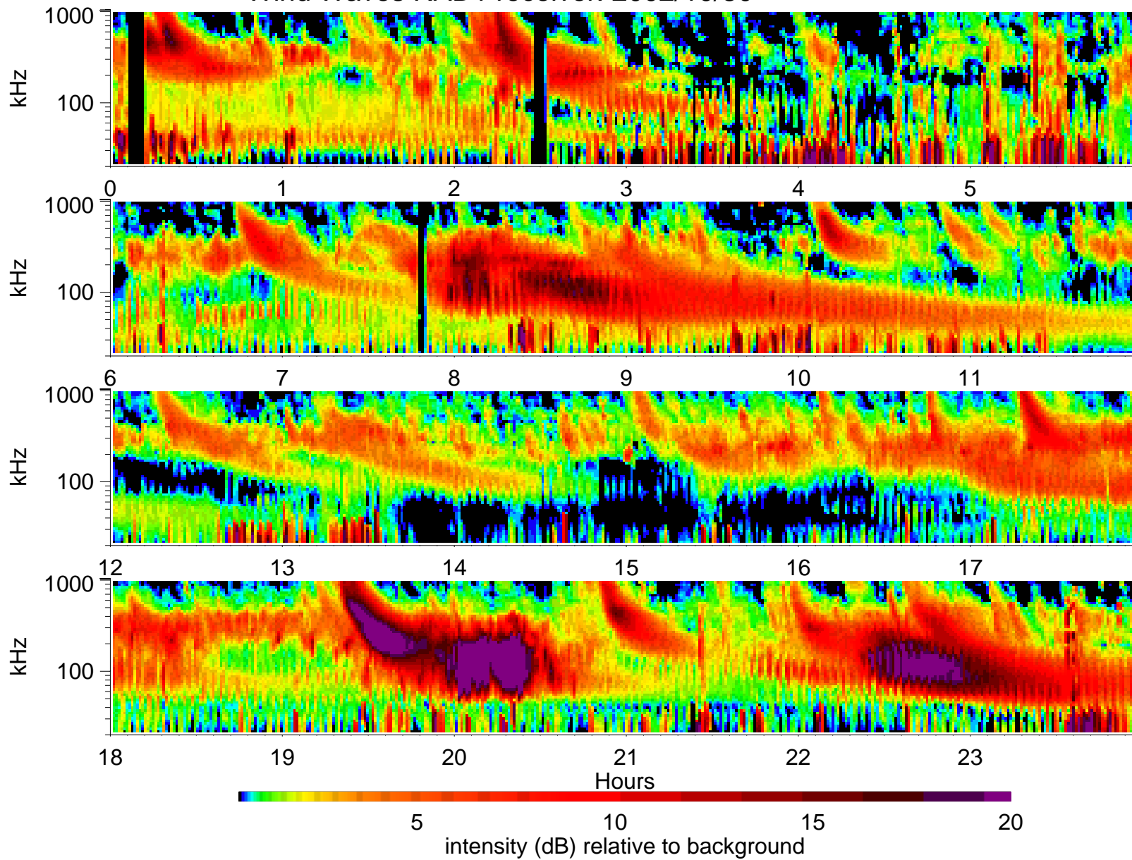
Wind Waves RAD1 receiver: 2002/10/30
