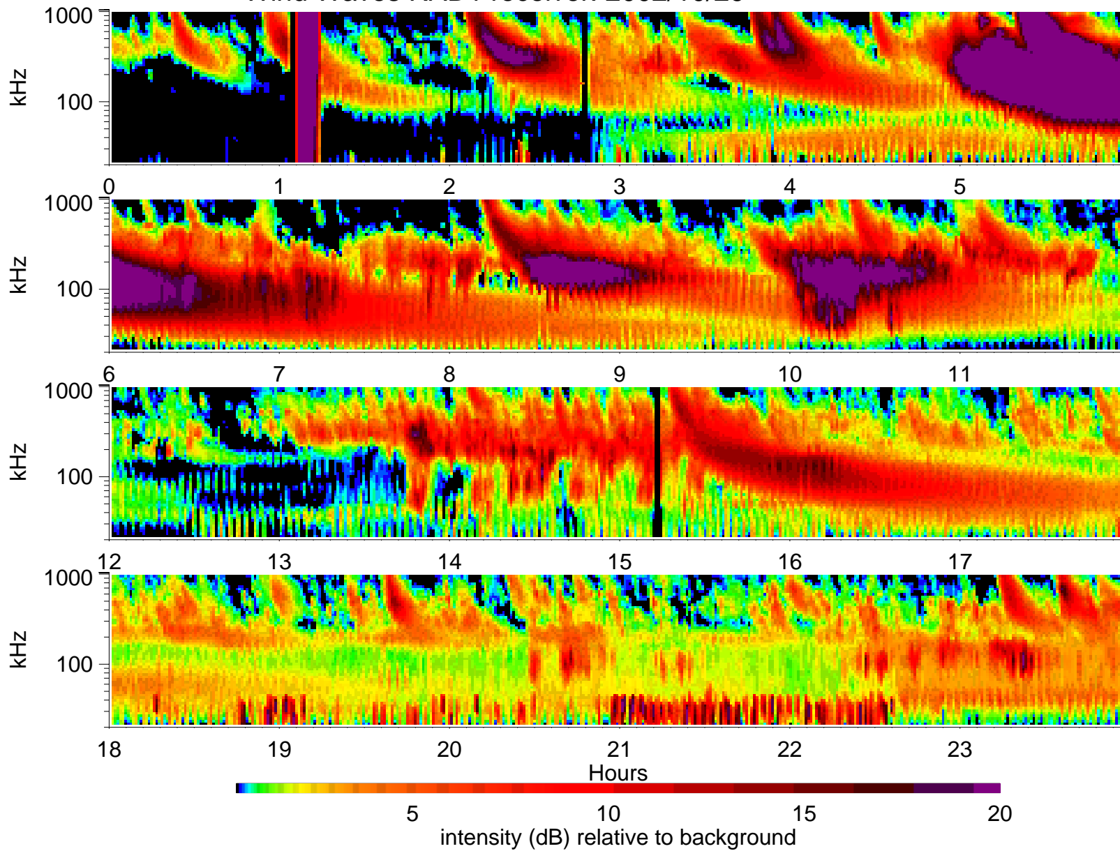
Wind Waves RAD1 receiver: 2002/10/29
