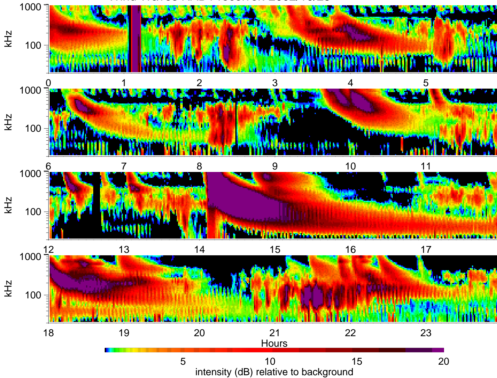
Wind Waves RAD1 receiver: 2002/10/25
