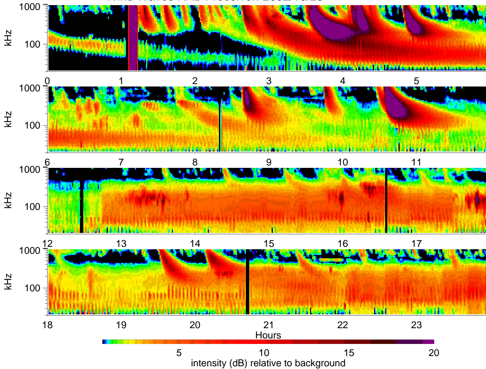
Wind Waves RAD1 receiver: 2002/10/23
