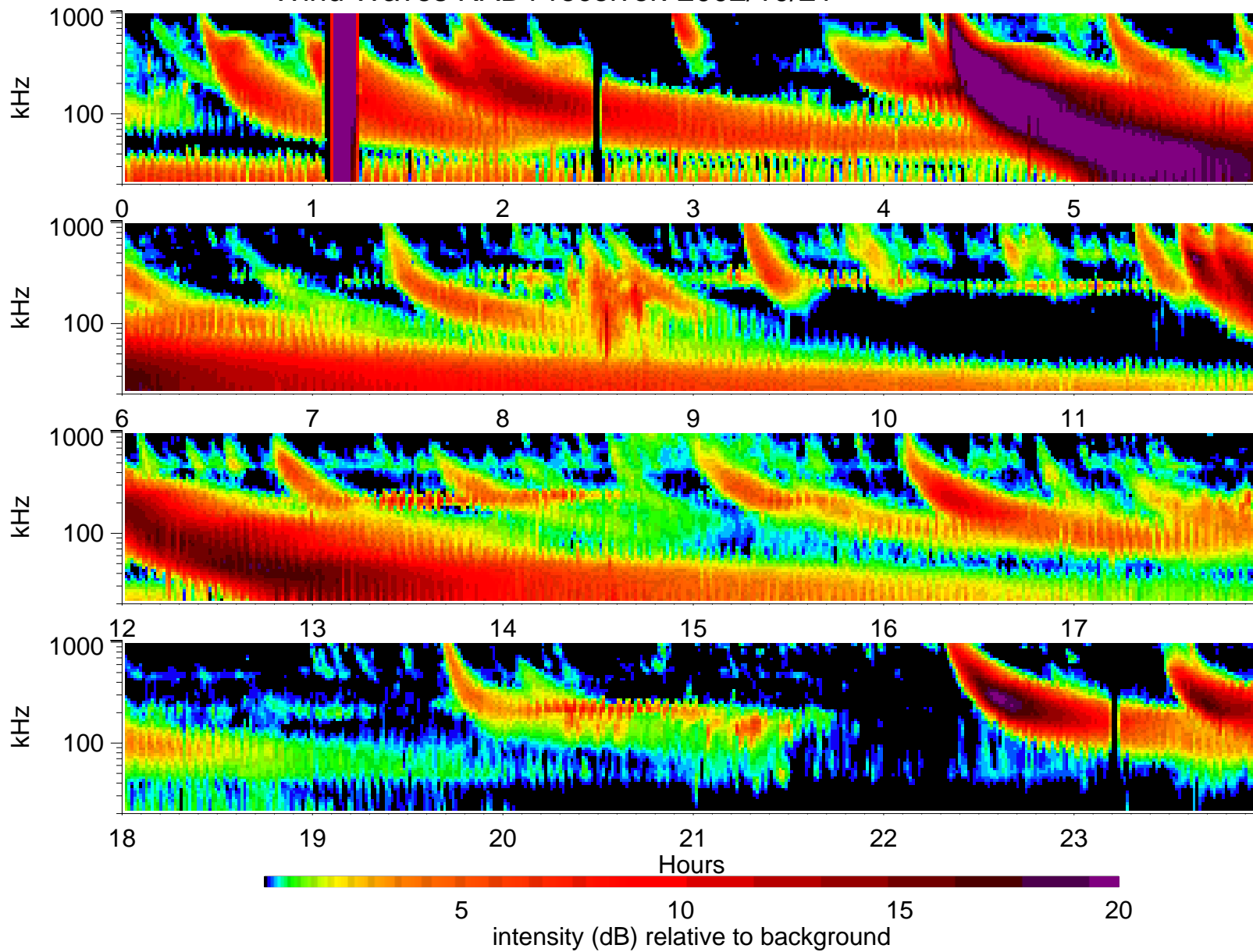
Wind Waves RAD1 receiver: 2002/10/21
