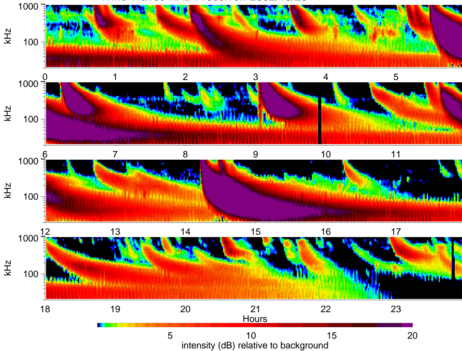
Wind Waves RAD1 receiver: 2002/10/20
