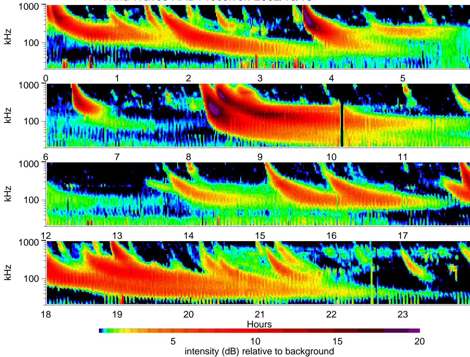
Wind Waves RAD1 receiver: 2002/10/18
