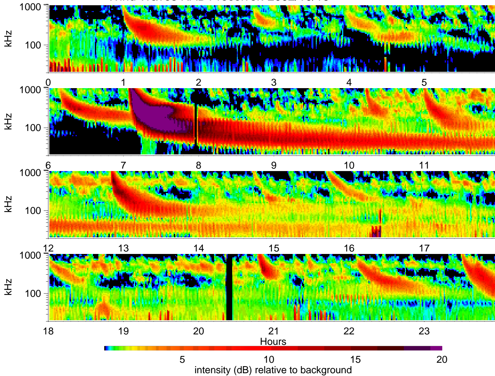
Wind Waves RAD1 receiver: 2002/10/16
