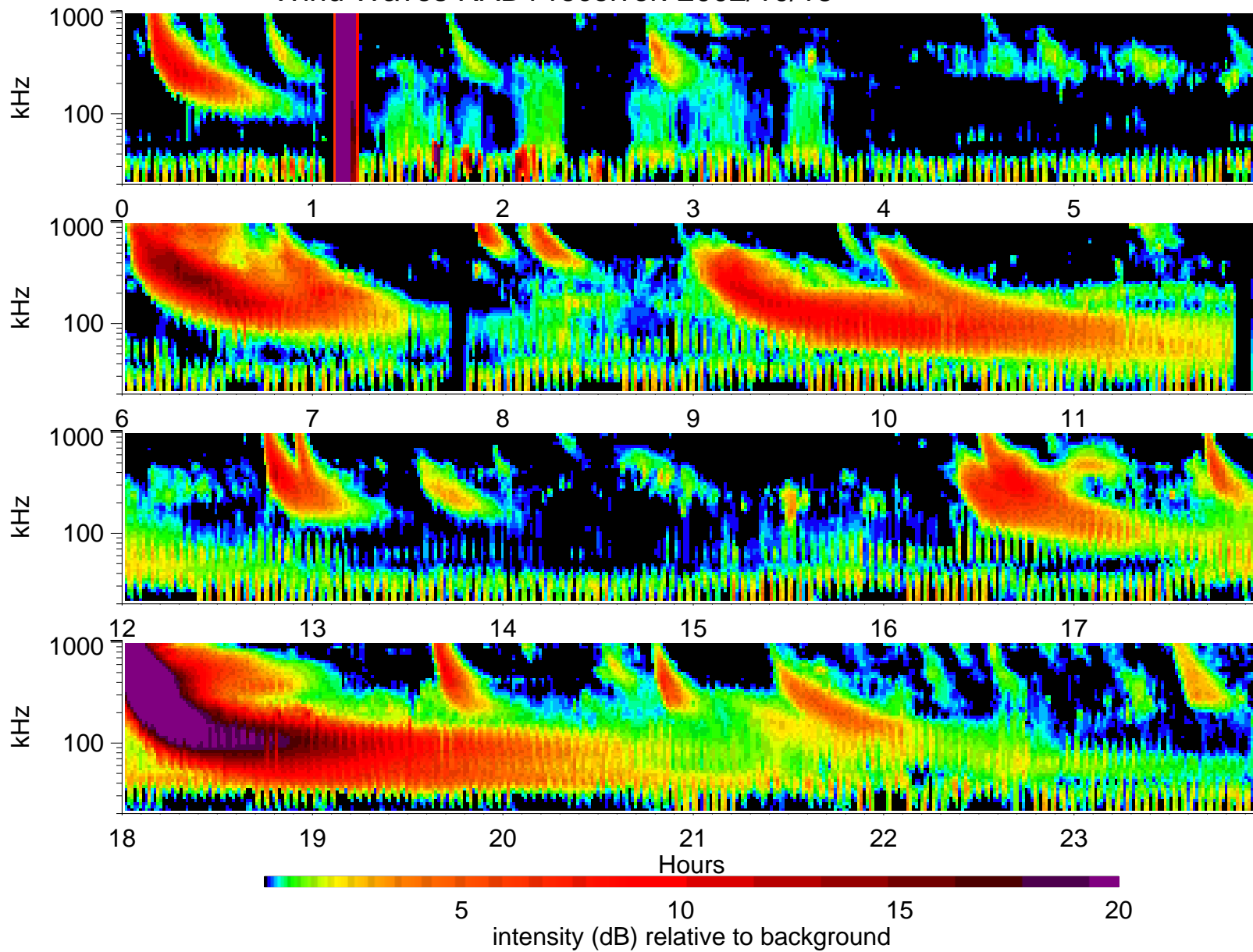
Wind Waves RAD1 receiver: 2002/10/13
