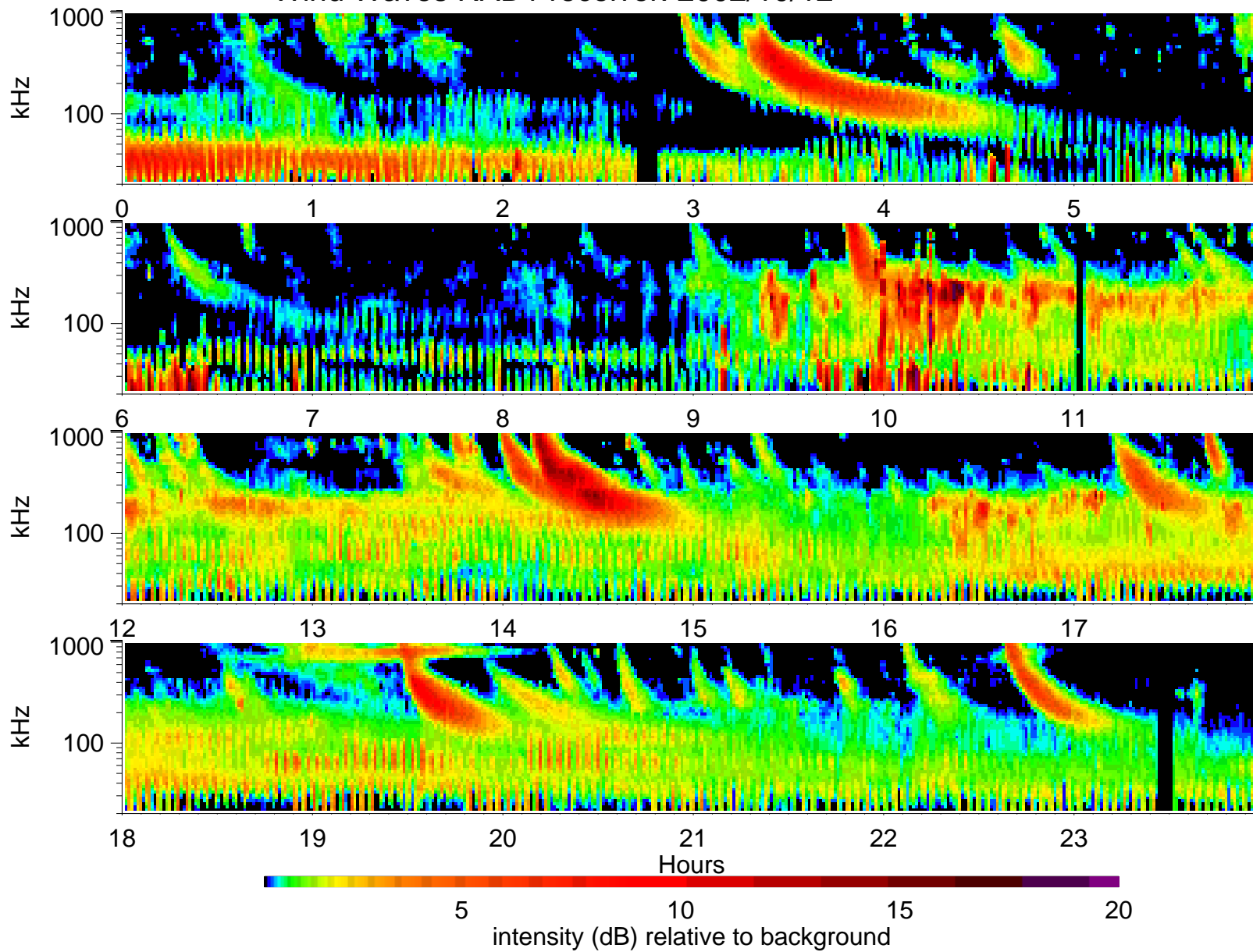
Wind Waves RAD1 receiver: 2002/10/12
