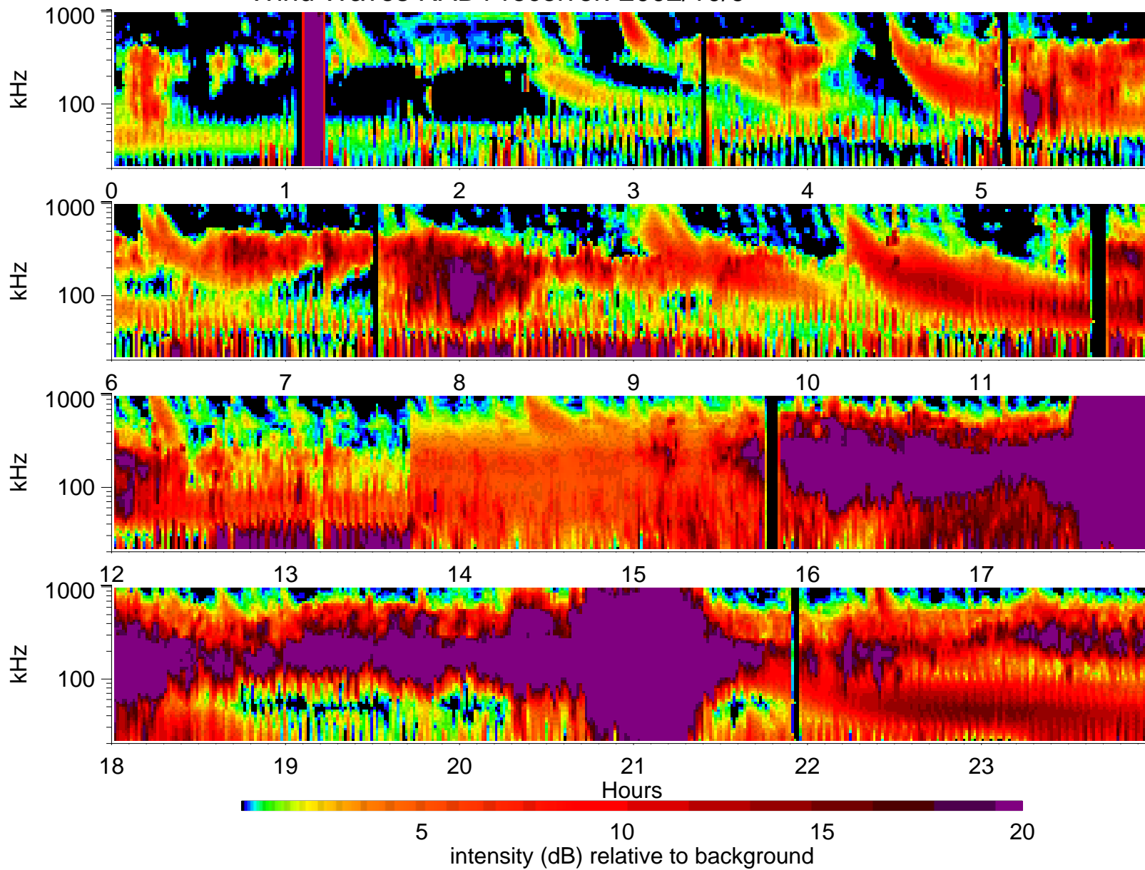
Wind Waves RAD1 receiver: 2002/10/9
