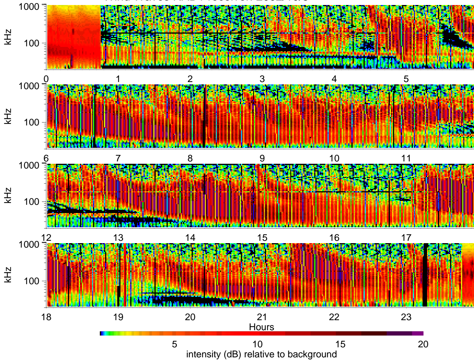
Wind Waves RAD1 receiver: 2002/10/8
