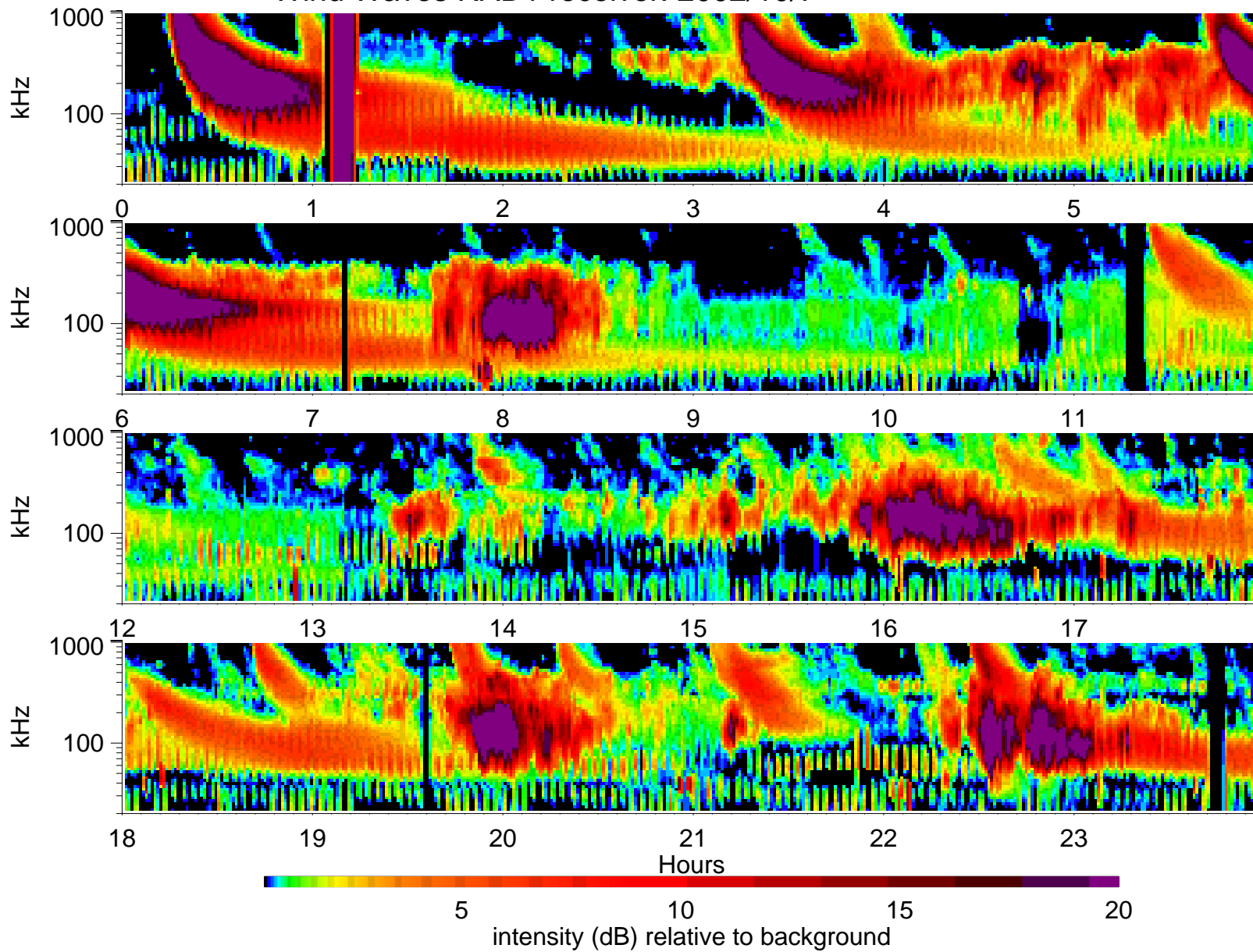
Wind Waves RAD1 receiver: 2002/10/7
