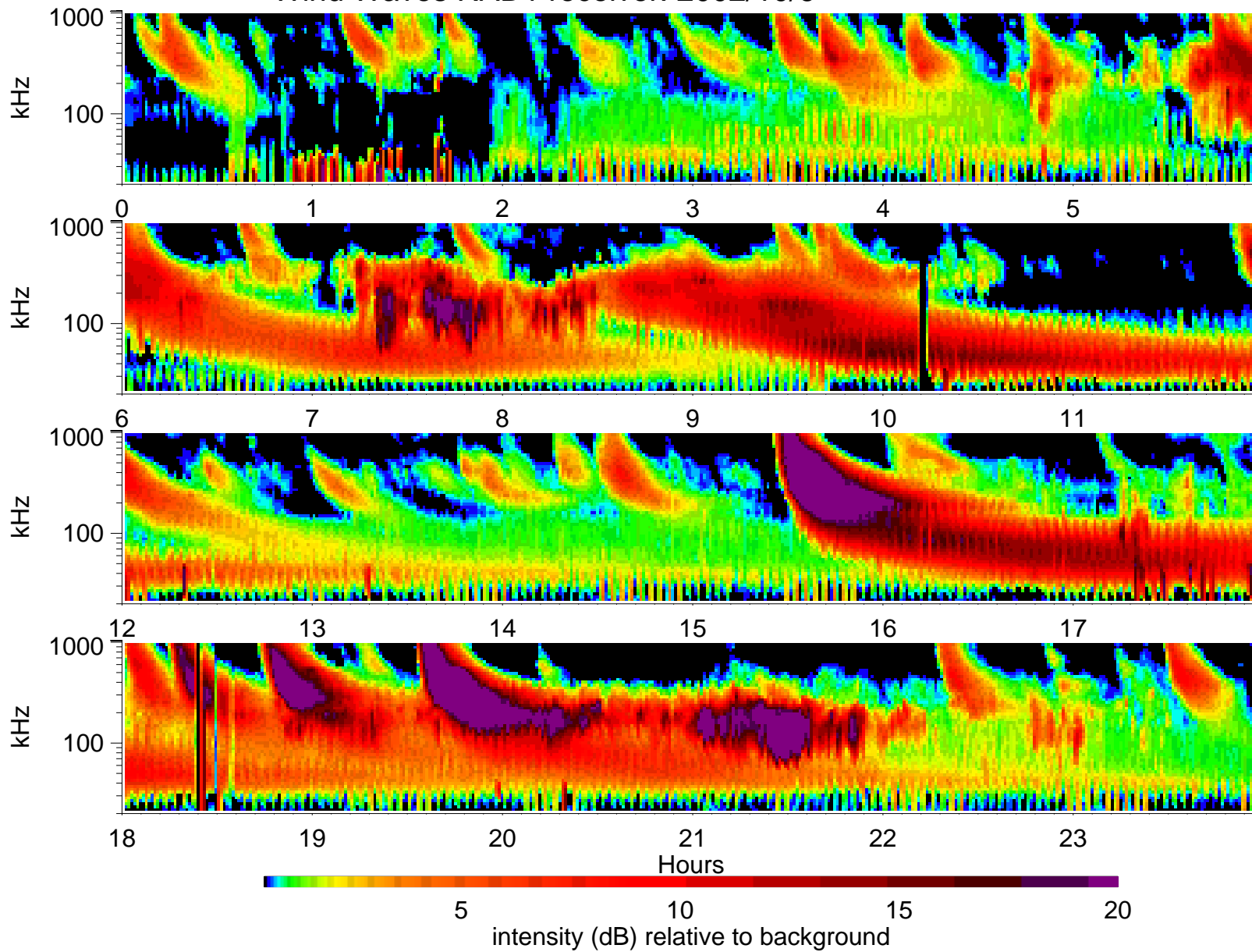
Wind Waves RAD1 receiver: 2002/10/6
