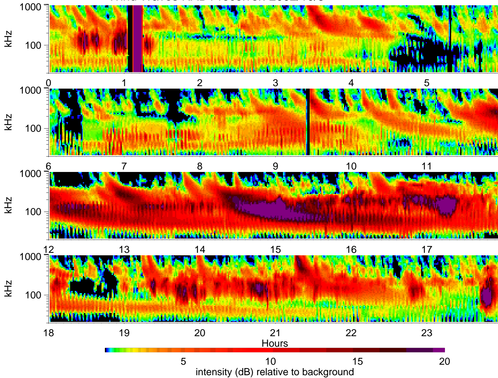
Wind Waves RAD1 receiver: 2002/10/3
