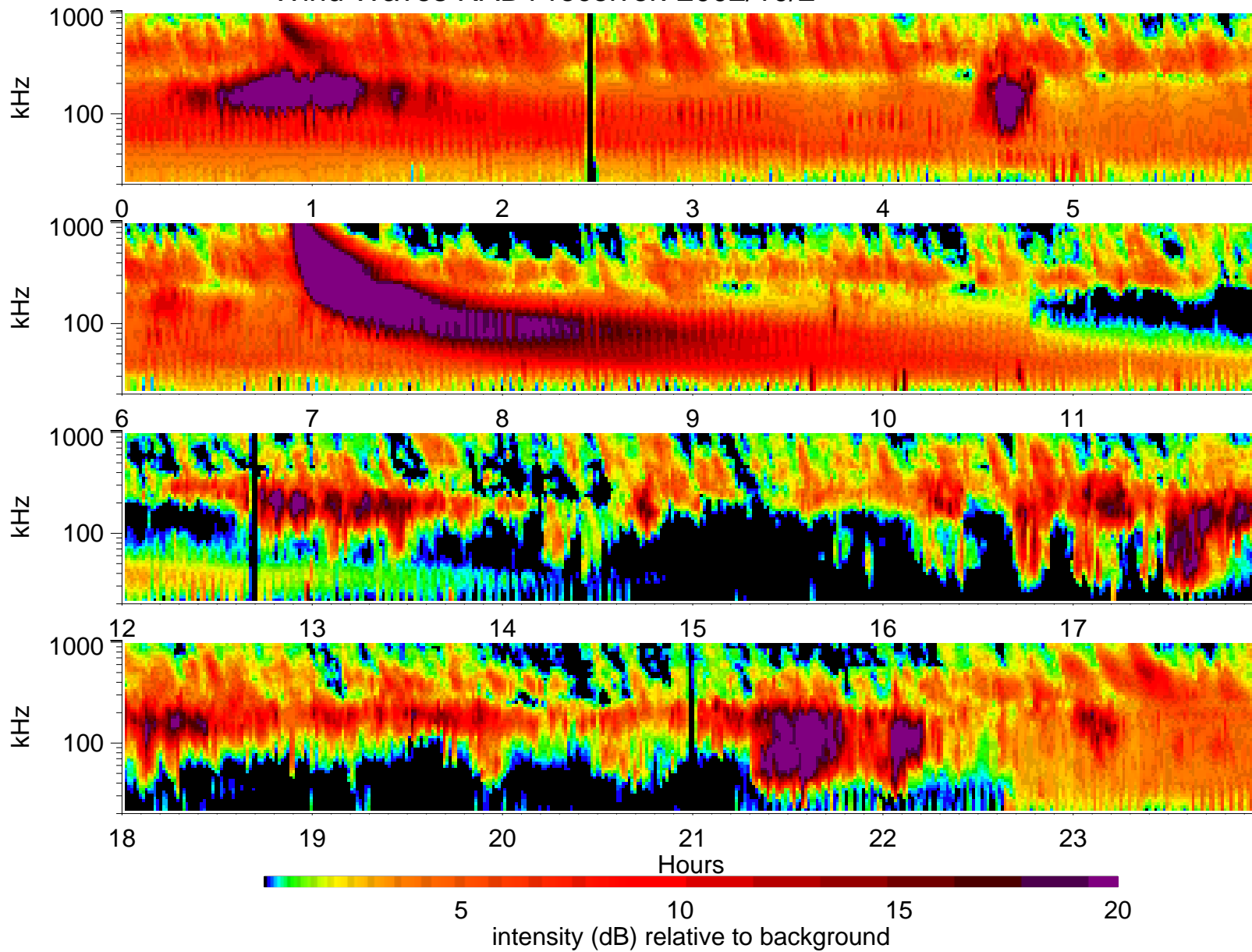
Wind Waves RAD1 receiver: 2002/10/2
