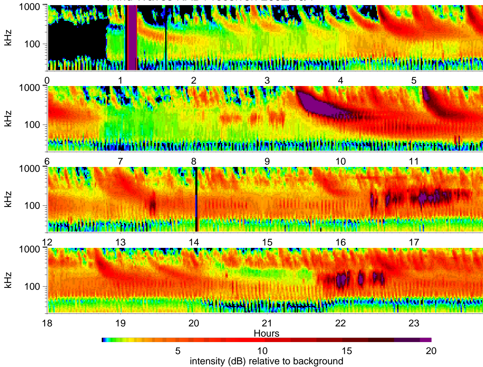
Wind Waves RAD1 receiver: 2002/10/1
