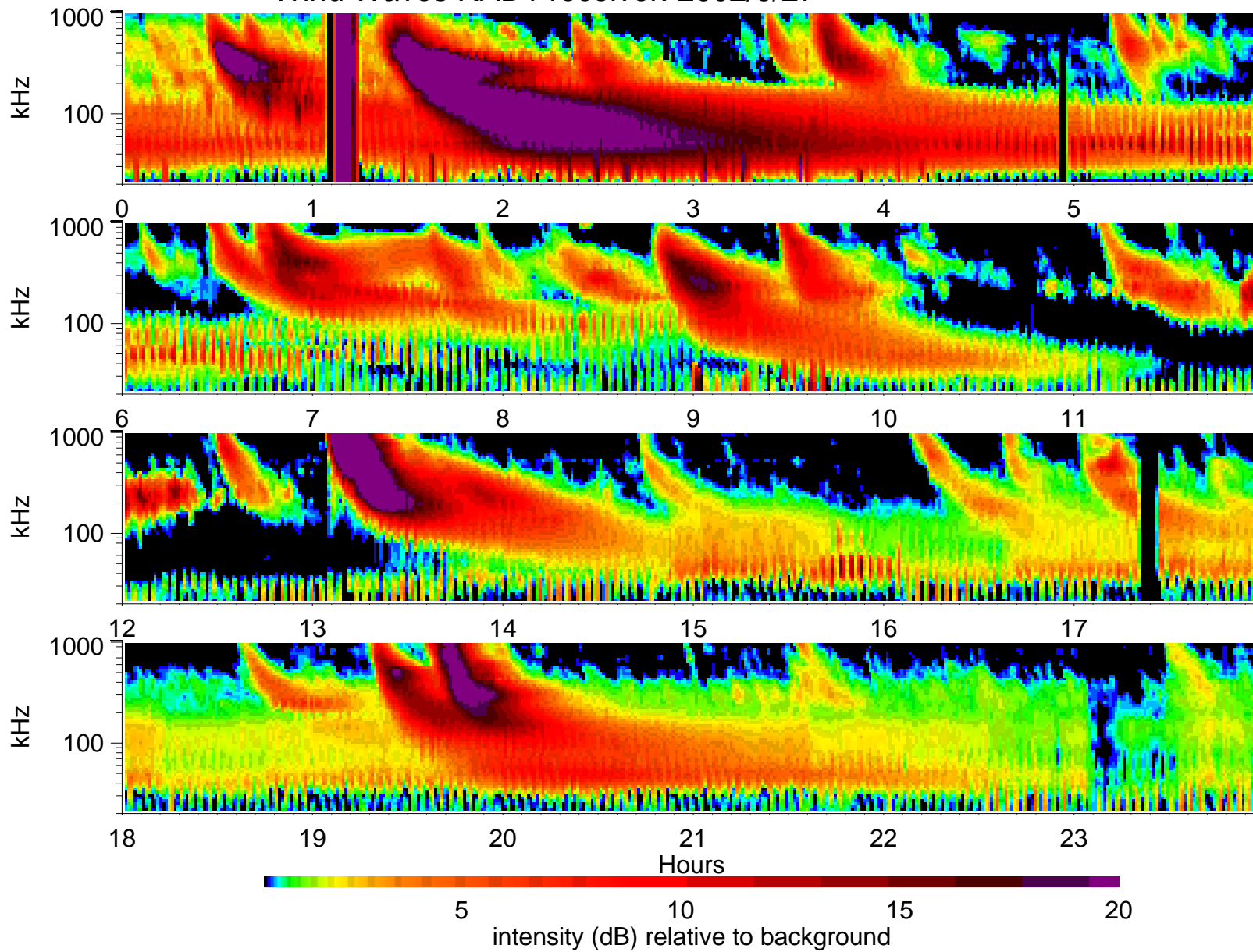
Wind Waves RAD1 receiver: 2002/9/27
