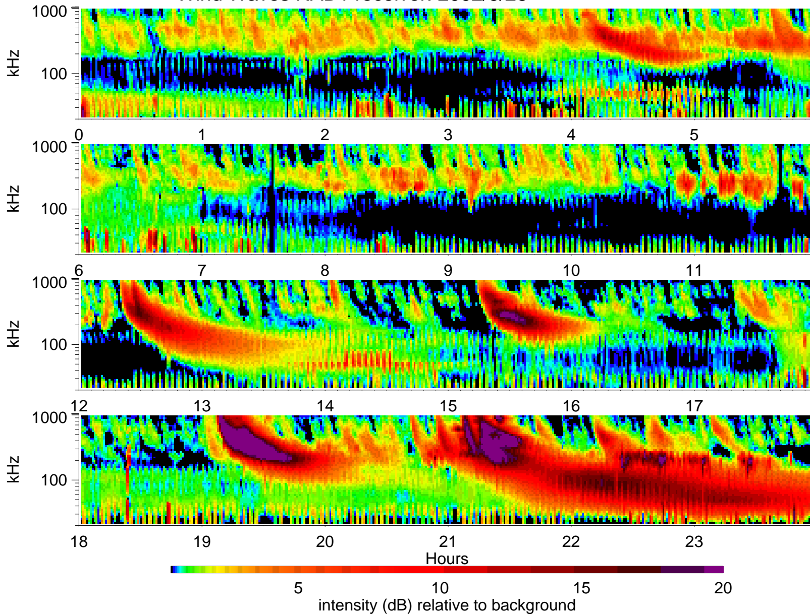
Wind Waves RAD1 receiver: 2002/9/26
