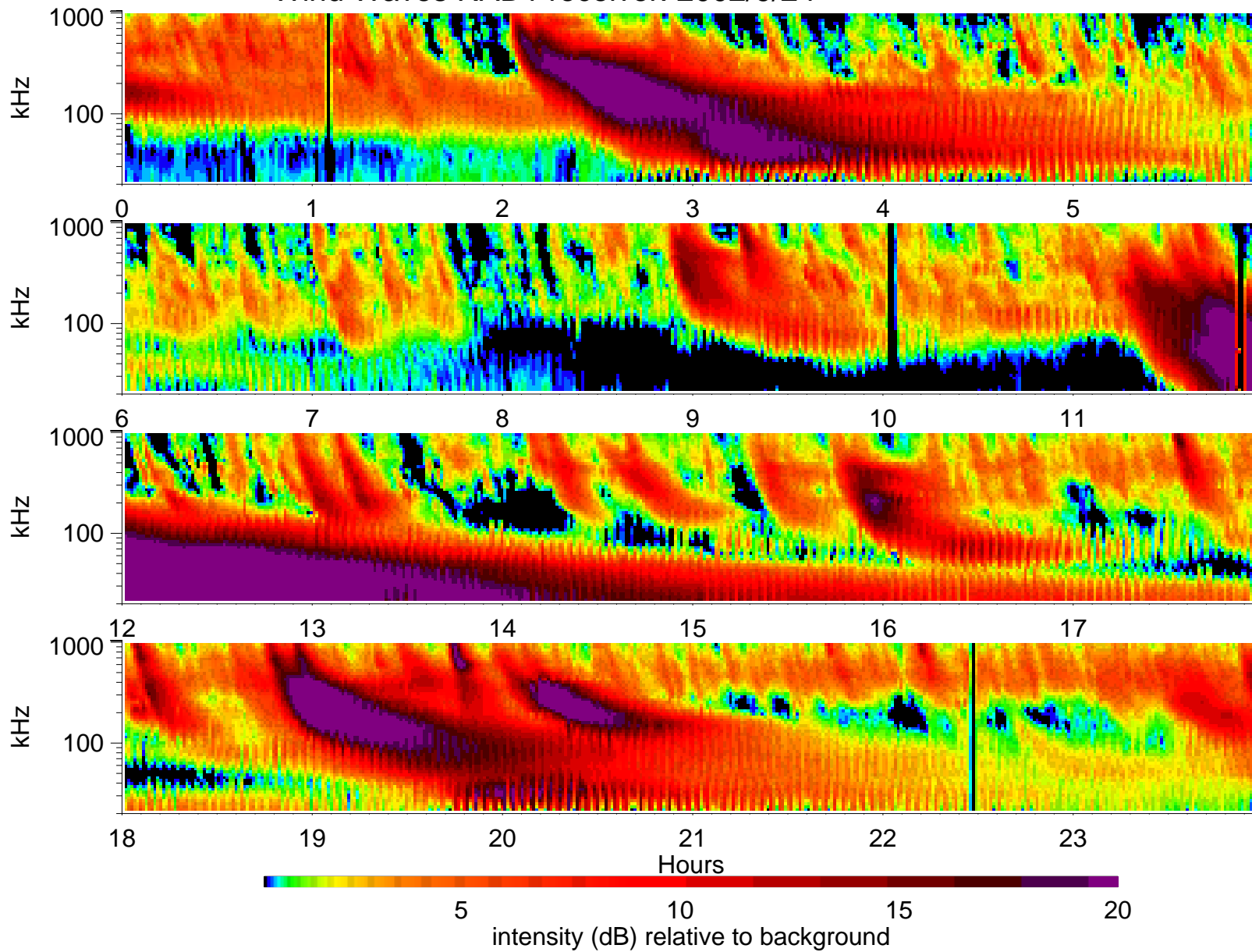
Wind Waves RAD1 receiver: 2002/9/24
