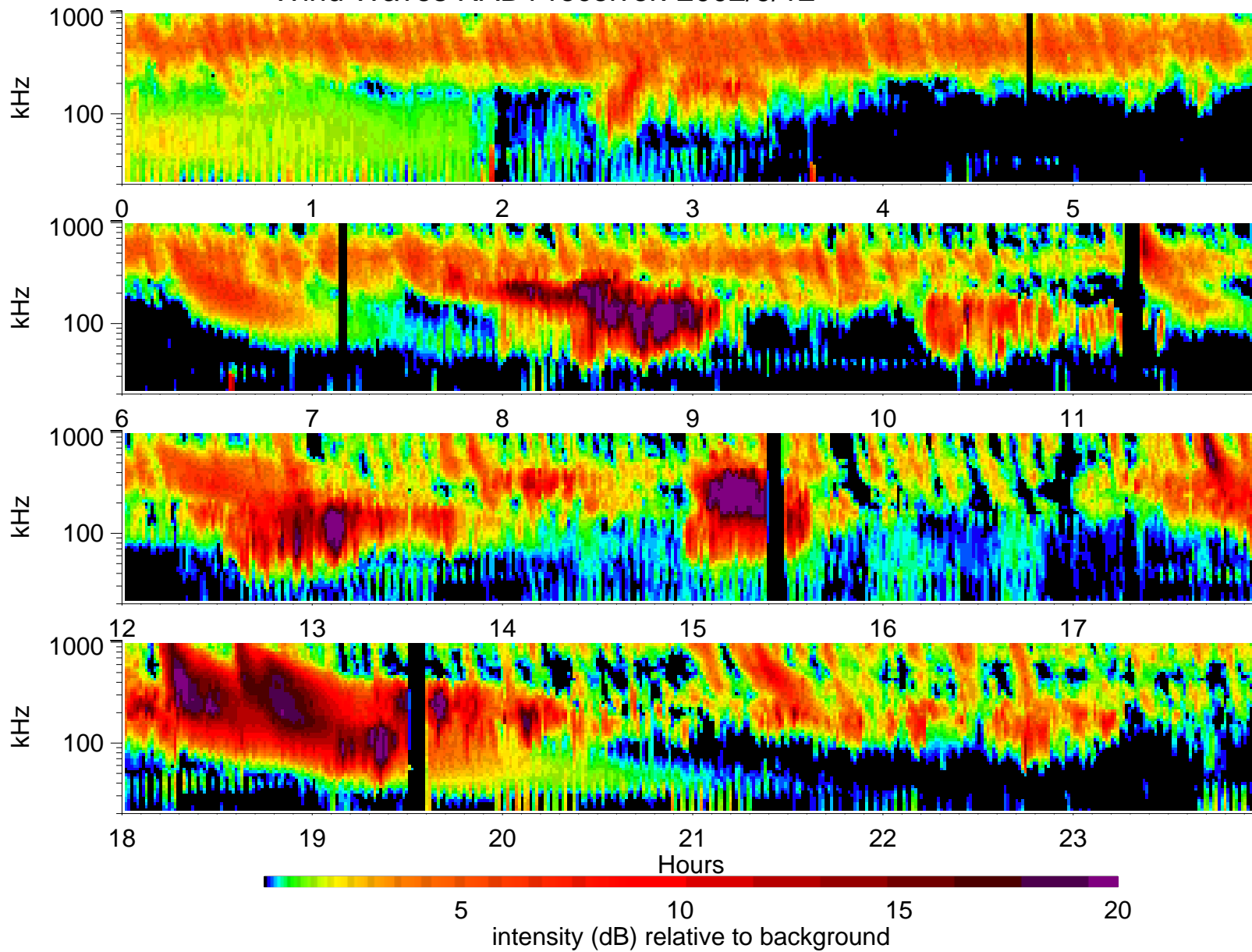
Wind Waves RAD1 receiver: 2002/9/12
