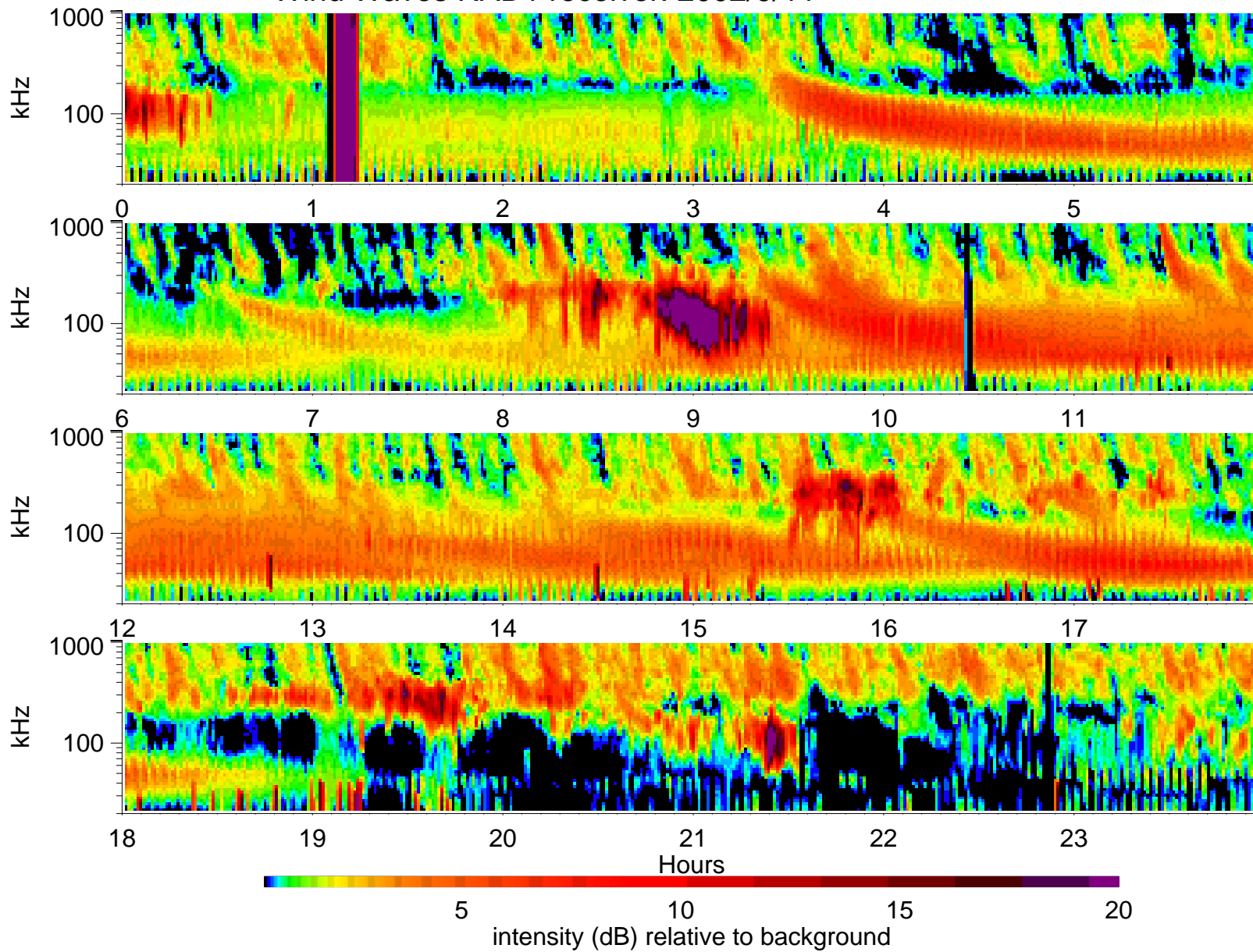
Wind Waves RAD1 receiver: 2002/9/11
