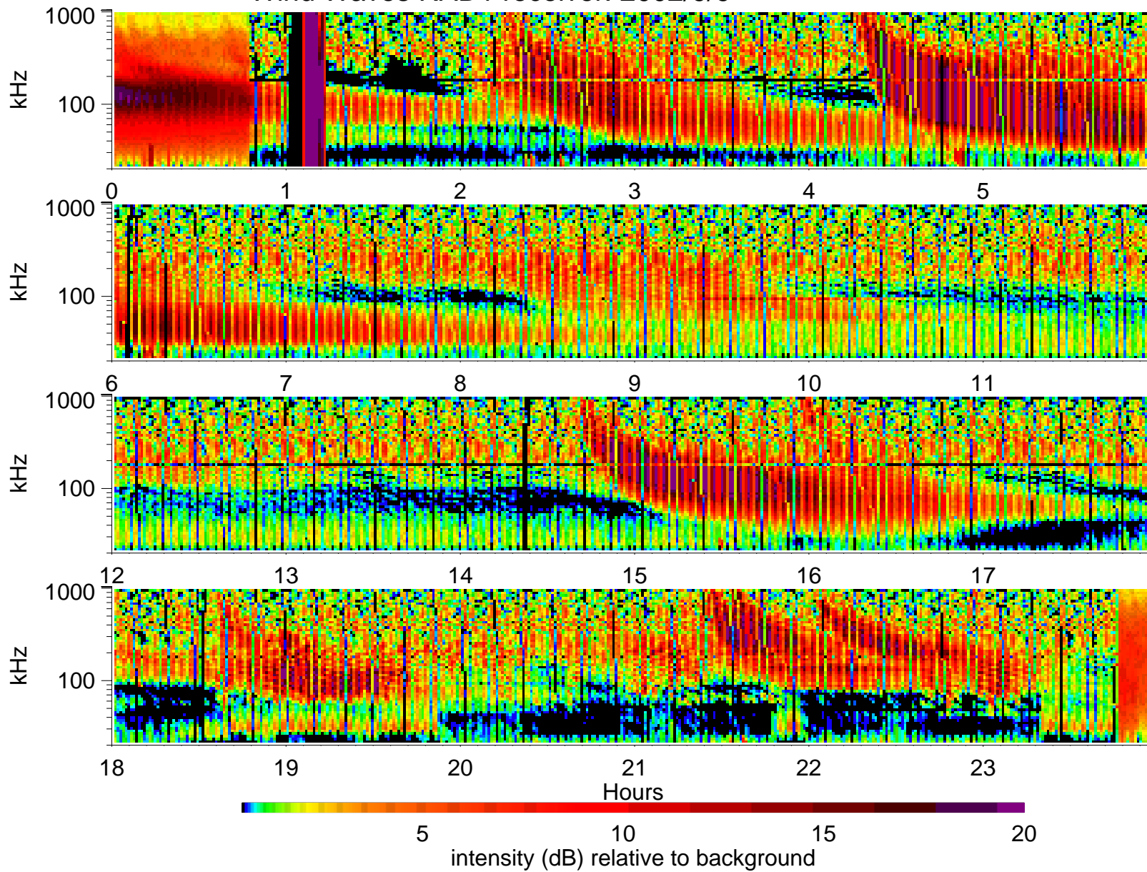
Wind Waves RAD1 receiver: 2002/9/9
