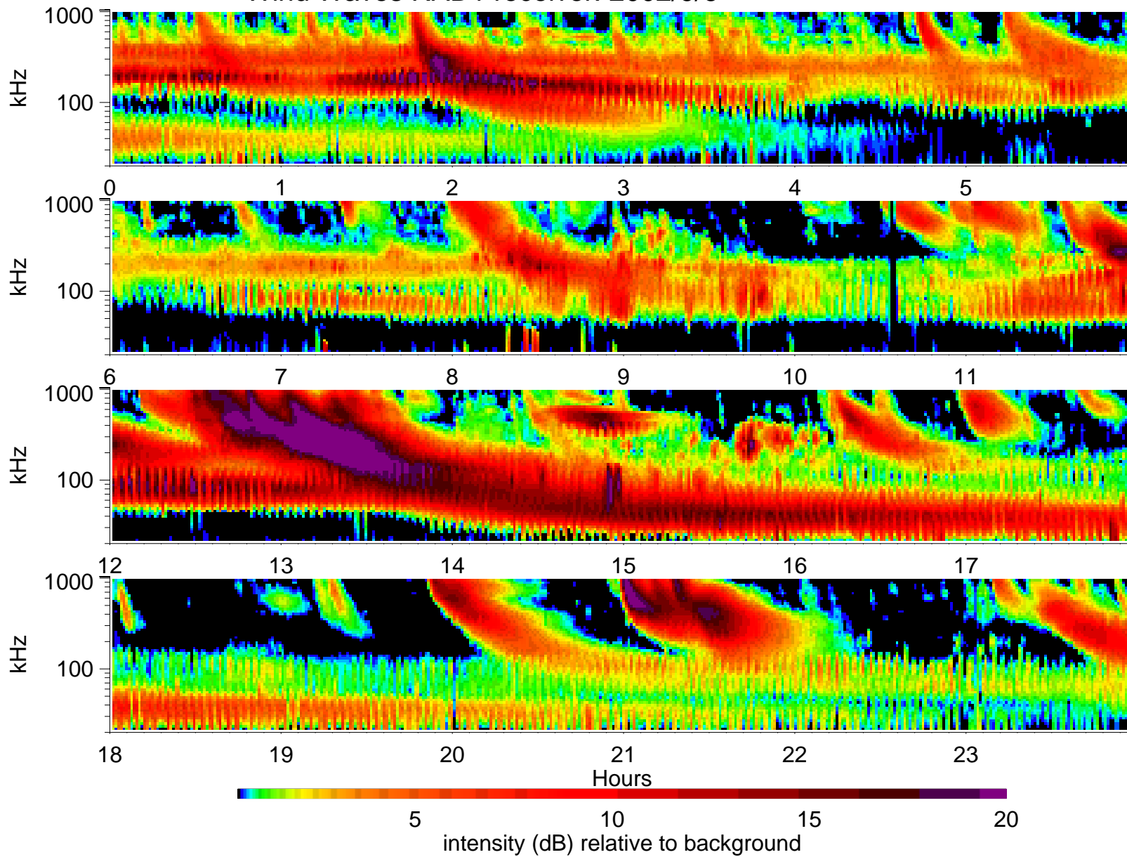
Wind Waves RAD1 receiver: 2002/9/6
