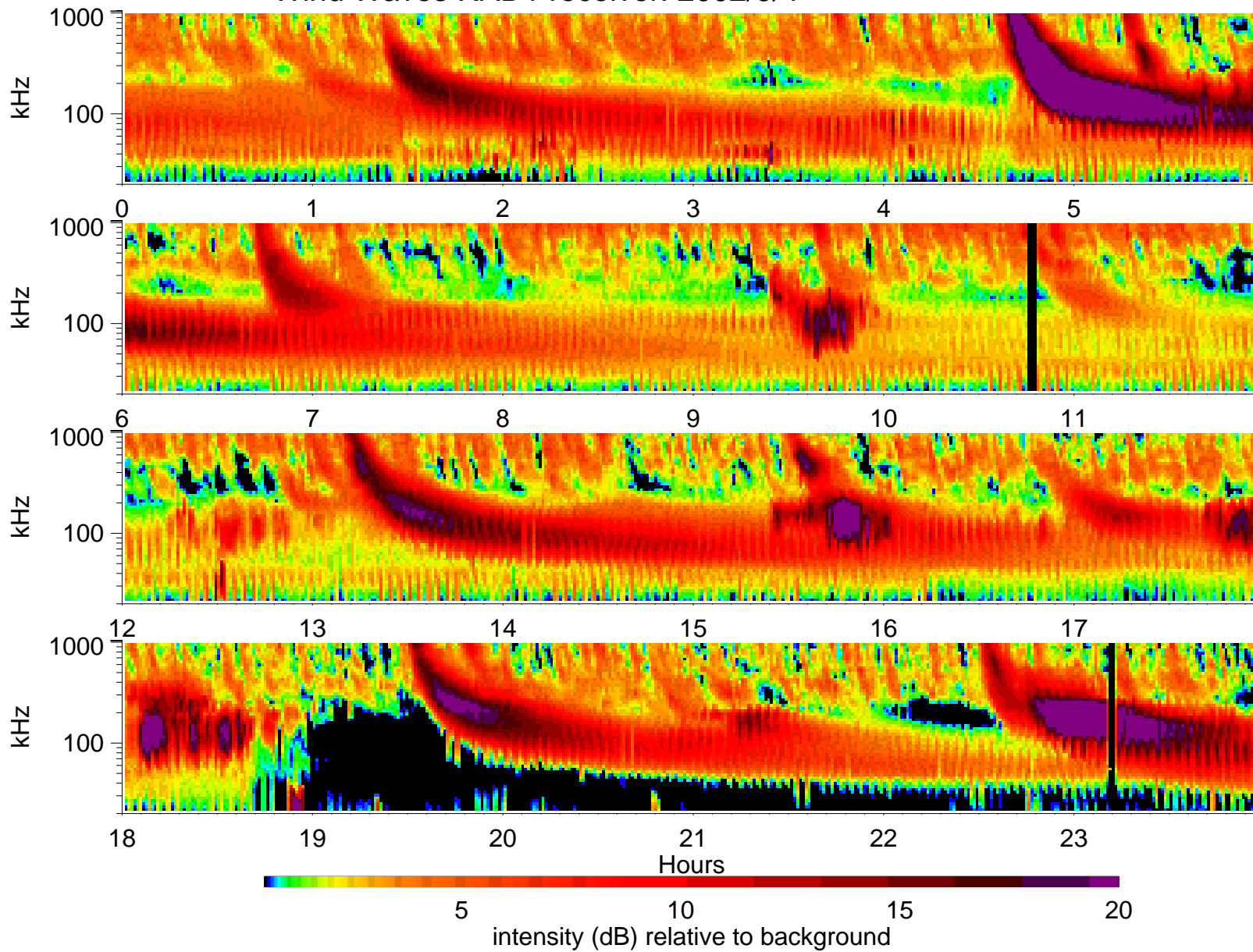
Wind Waves RAD1 receiver: 2002/9/4
