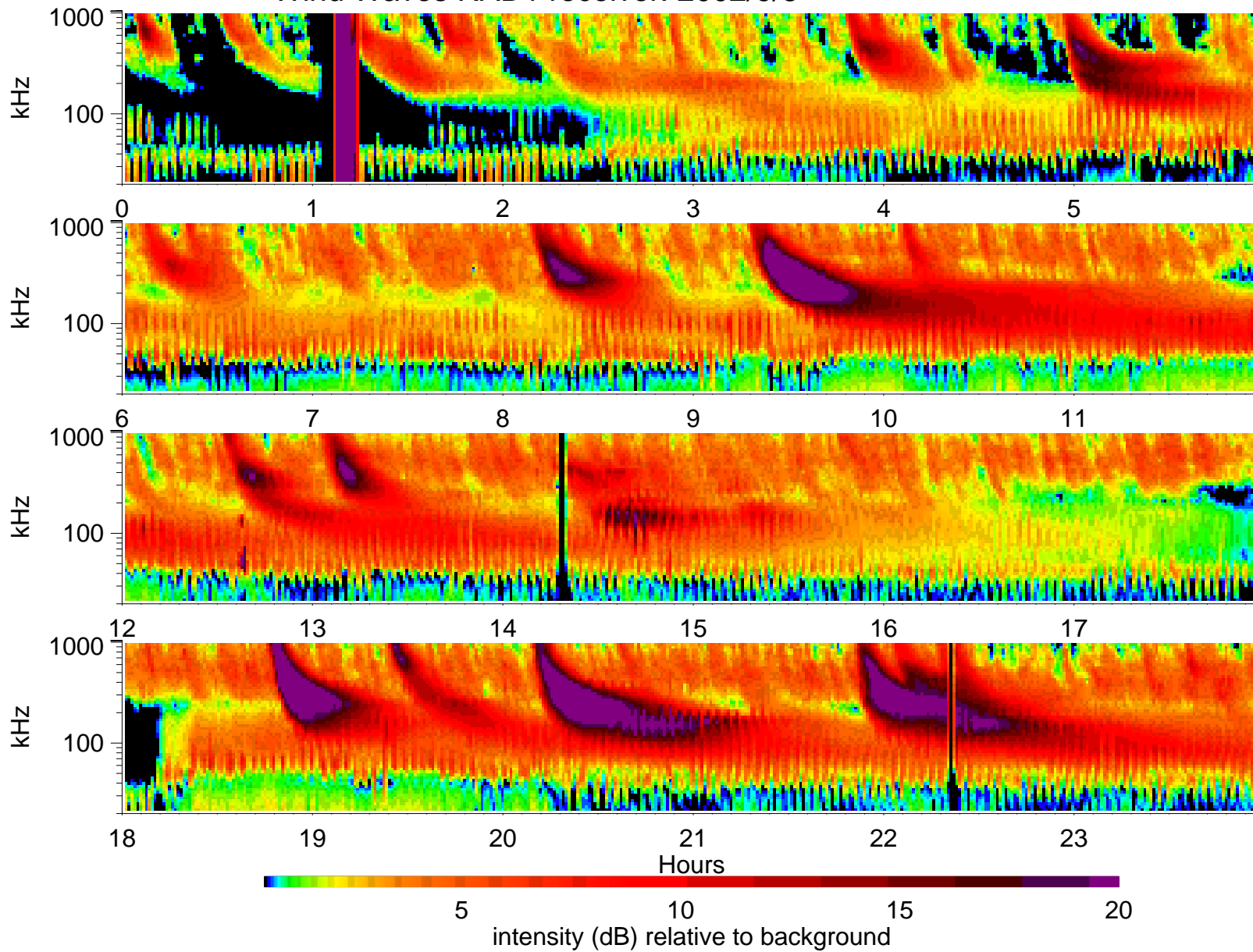
Wind Waves RAD1 receiver: 2002/9/3
