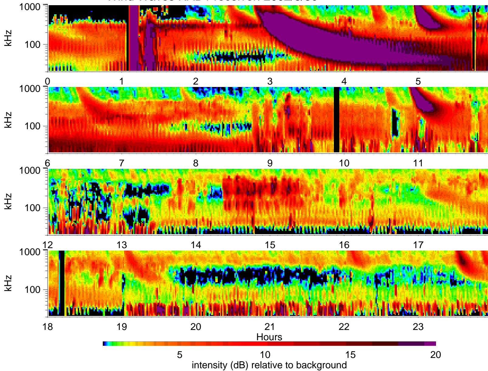
Wind Waves RAD1 receiver: 2002/8/30
